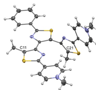
Figure 1. An ORTEP drawing of 2o 2+ . Thermal ellipsoids are shown at the 30% level. Anions and solvent molecules are omitted for clarity. Deposition number 2084834 contains the supplementary crystallographic data for this paper. These data are provided free of charge by the joint Cambridge Crystallographic Data Centre and Fachinformationszentrum Karlsruhe Access Structures service.
