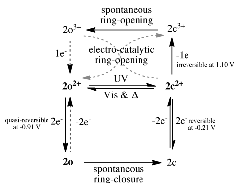
Scheme 3. Photochemical and electrochemical transformation between 2o^{2+} and 2c^{2+} .
