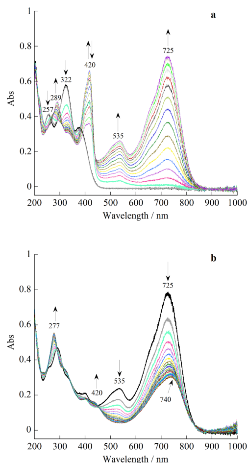
Figure 5. Absorption spectral changes of 2\mathbf{o}^{2+} ( 1.75 \cdot 10^{-4} M) during electrolysis (a) at -1.10 V and then (b) at 0.0 V (vs SCE) in 0.2 M \text{Bu}_4\text{NPF}_6/\text{MeCN} at -25 °C.
