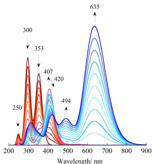
Figure 10. Calculated absorption spectral evolution of the reduction of 2\mathbf{o}^{2+} to the neutral 2\mathbf{o} and then the spontaneous ring-closure to the neutral 2\mathbf{c} .
