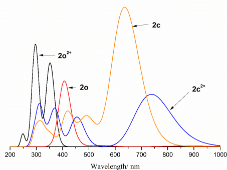
Figure 9. Calculated electronic spectra of 2\mathbf{o}^{2+} , 2\mathbf{c}^{2+} , 2\mathbf{o} and 2\mathbf{c} .
