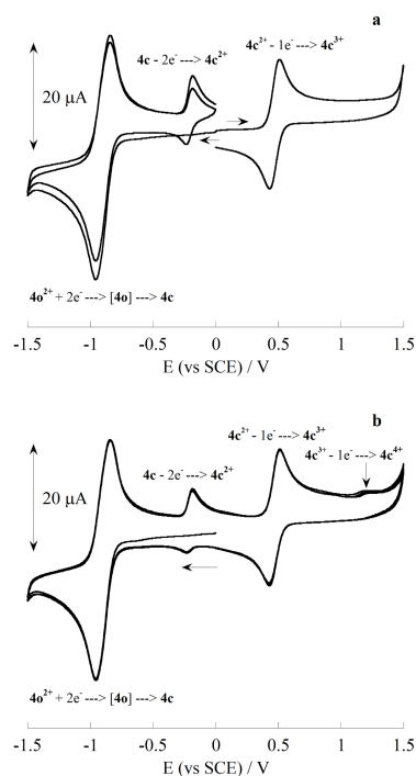
Figure 4. Cyclic voltammograms of 4o 2+ (1.0 mM) in MeCN containing 0.10 M Bu 4 NPF 6 at 20°C, v = 0.1 Vs -1 : a) reductive cyclization and reversible oxidation of the ferrocenyl moiety; b) reductive cyclization and oxidative ring-opening.
