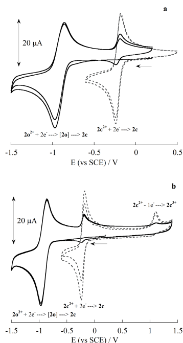
Figure 3. Cyclic voltammograms of 2o 2+ (plain plots) (1.0 mM) in MeCN containing 0.10 M Bu 4 NPF 6 at 20°C, v = 0.1 Vs -1 and those of its UV irradiated solution (dotted plots): a) reductive cyclization; b) reductive cyclization and oxidative ring-opening.
