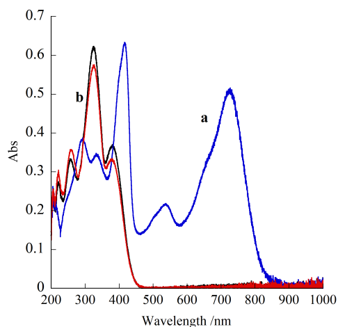
Figure 6. Absorption spectra of 2o^{2+} ( 1.75 \cdot 10^{-4} M) (black) after electrolysis (a) at -1.10 V (blue) and then (b) at 1.40 V (red) (vs SCE) in 0.2 M Bu_4NPF_6/MeCN at -25^\circ C .
