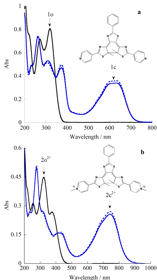
Figure 2. Absorption spectra of 1\mathbf{o} ( 2.66 \times 10^{-5} M in 1 cm cell) (a) and 2\mathbf{o}^{2+} ( 1.55 \times 10^{-4} M in 1 mm cell) (b) in MeCN at RT along with their photo-stationary state (PSS, solid blue line) at 320 and 365 nm, respectively, and the calculated spectra of their respective closed form (dotted blue line).
