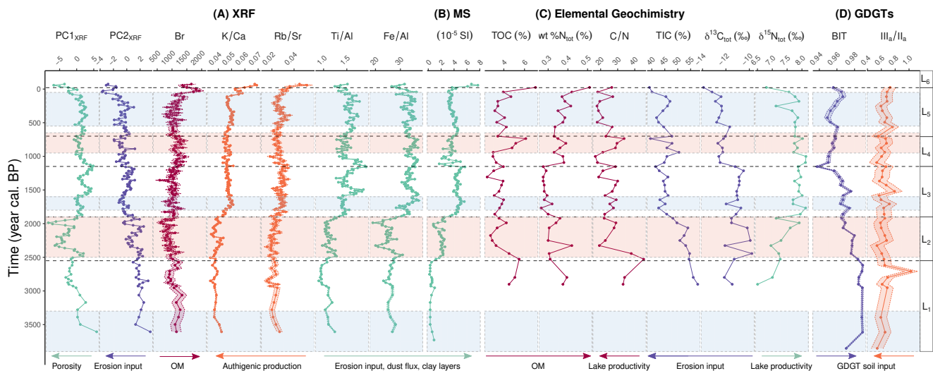
Figure 4: Geochemistry proxies applied to the Lake Ayrag sequence. A: selected XRF signals ( PC_1 and PC_2 from Fig. 3, ratio of Potassium / Calcium, Rubidium / Strontium, Titanium / Aluminum, Iron / Aluminum); B: magnetic susceptibility; C: selected isotopes and element mass abundances (Total Organic Carbon (TOC), weight percentage of bulk Nitrogen ( w\%N_{tot} ), Total Inorganic Carbon (TIC), the ratio between TOC and w\%N_{tot} (C/N), bulk \delta^{13}C , bulk \delta^{15}N ); D: GDGT index for source origin (branched vs. isoprenoid tetraether (BIT) index and ratio III_a/II_a ). Colors highlight the signals following the same trend: green curves show sediment compaction, and the clay and dust inputs provide nutrients for increasing lake productivity; purple curves decrease with lithogenic and ex-situ OM input, soil brGDGT, and algal production; purple curves show OM amount in the sediment; orange curves decrease with authigenic production.
