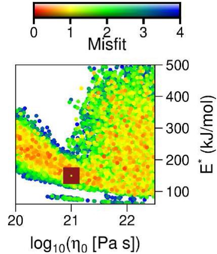
Figure A1. Inversion results using both body waves and surface waves arrival times, considering that V^* can vary between 0 and 7\text{ cm}^3\text{ mol}^{-1} . The figure shows \eta_0 as a function of E^* , for all the models accepted by the Bayesian algorithm (coloured dots). Red and blue colours indicate small and large misfit values, respectively. The dark red square corresponds to the values to retrieve ( \eta_0 = 10^{21}\text{ Pa s} and E^* = 150\text{ kJ mol}^{-1} ).
