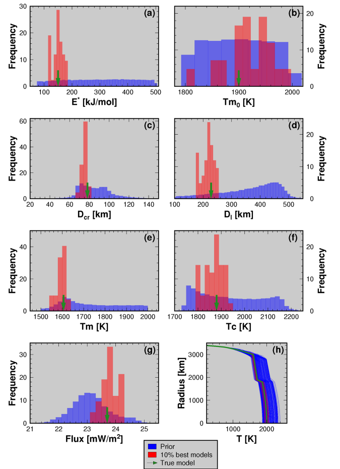
Geodynamically-constrained inversion: four events (body waves only)
