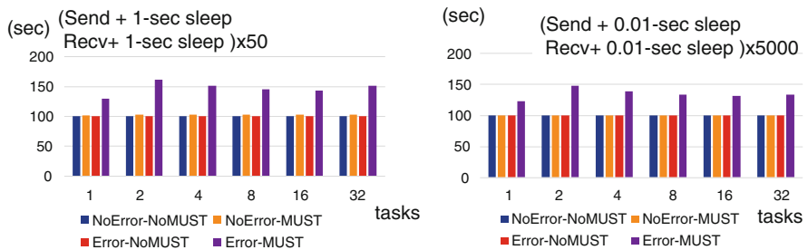
Fig. 23 Execution time when a workflow includes 1, 2, ... 32 tasks executing MPI_Send/Recv repeatedly every 1-s (left) and every 0.01-s
