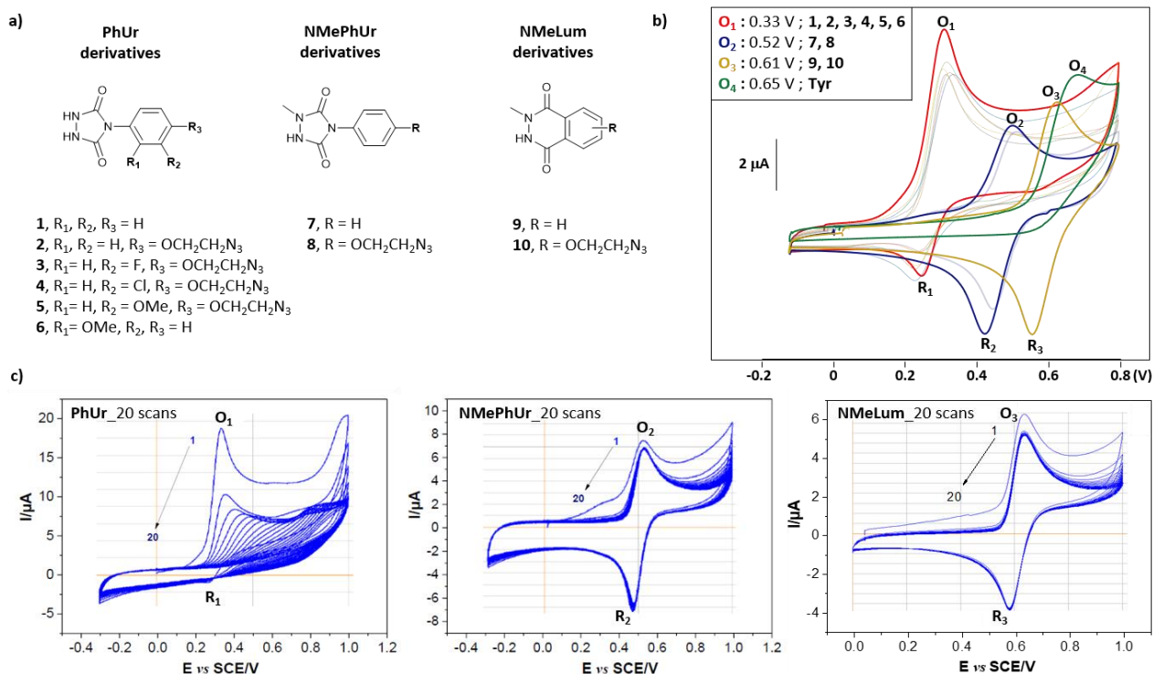
Fig. 2 Electrochemical behaviour of the studied Y anchors PhUr 1-6, NMePhUr 7, 8 and NMeLum 9, 10. a) Chemical structures of the compounds 1-10, b) Cyclic voltammetry of 1-10 and Y (cathode: graphite carbon electrode 2 mm disc, anode: platinum wire, reference: saturated calomel electrode, 100 mV/s, reagent 1 mM, 1:1 MeCN/Tris 50 mM pH 7.4), c) Multicyclic voltammetry of 1, 7 and 9 (cathode: graphite carbon electrode 2 mm disc, anode: platinum wire, reference: saturated calomel electrode, 100 mV/s, reagent 1 mM, 1:1 MeCN/NH 4 OAc 100 mM pH 7.4).
