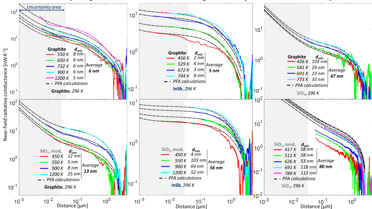
Fig. A.7: Experimental estimation of the minimum distance before contact. Near-field radiative conductance calculations using PFA are compared with measurements after fitting and adjusting the distance scale.
