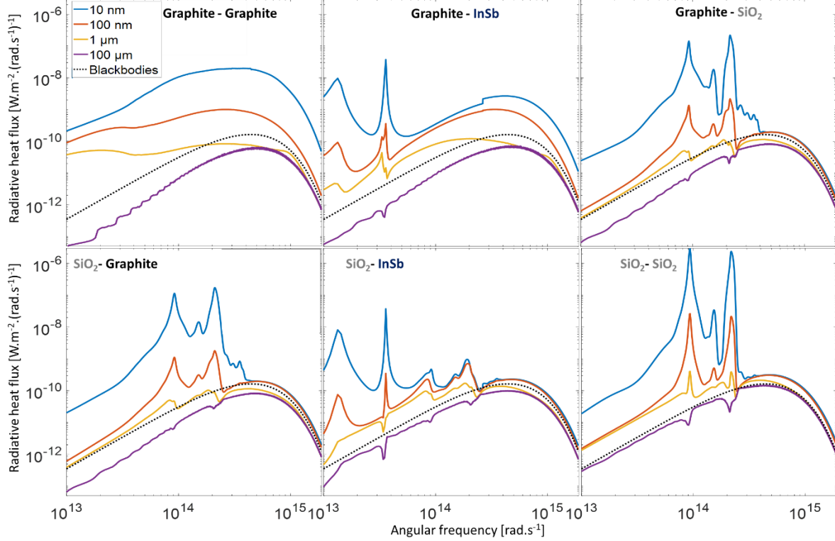
Fig. A.9: Radiative heat flux as a function of angular frequency between planar bodies at 1200 K, made of graphite or \text{SiO}_2 , and planar bodies at 300 K made of either graphite, InSb or \text{SiO}_2 .
