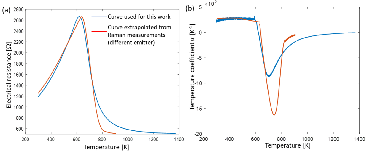
Fig. A.10: Comparison of two emitter calibration methods. (a) Electrical resistance as a function of temperature. The blue curve shows the calibration curve used for this work and obtained using the method described in section A.2. The red curve corresponds to a calibration curve extrapolated from Raman temperature measurements performed on another emitter. (b) Temperature coefficients calculated from the two calibration curves.
