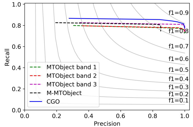
FIGURE 14: Evaluation on the FDS Simulation.
