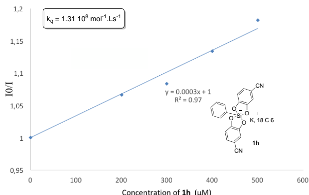
Figure 5. Stern-Volmer plot - quench of silicate 1h and 3
