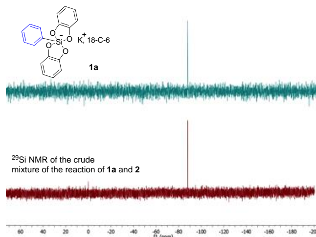
Figure 1. 29 Si NMR monitoring of the photocatalytic reaction of 1a with 2a in DMF-d 7 .
