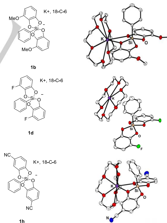
Figure 2. XRD analyses of silicates 1b , 1d and 1h . Only cis isomer of 1d depicted and hydrogens omitted for clarity.
