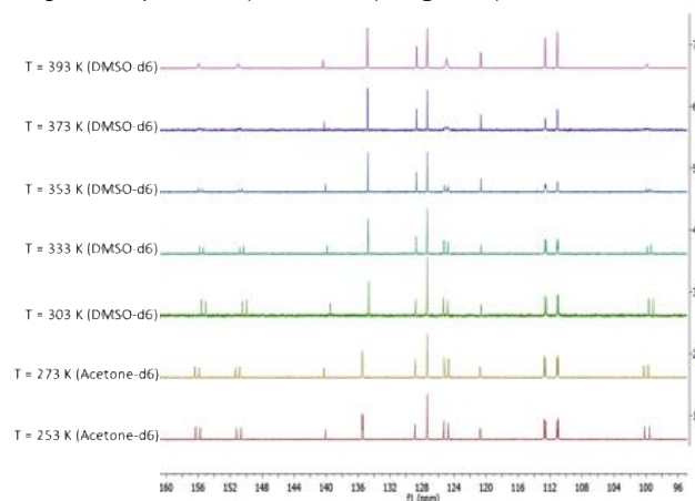
Figure 3. ^{13}\text{C} NMR of silicate 1h at various temperatures
