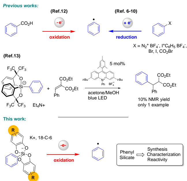
Scheme 2. Generation of aryl radicals through photocatalytic conditions
