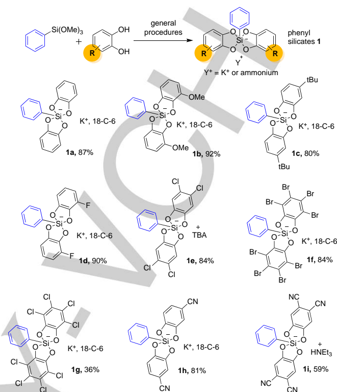
Scheme 5. Preparation of phenyl silicates 1 bearing substituted catechols
