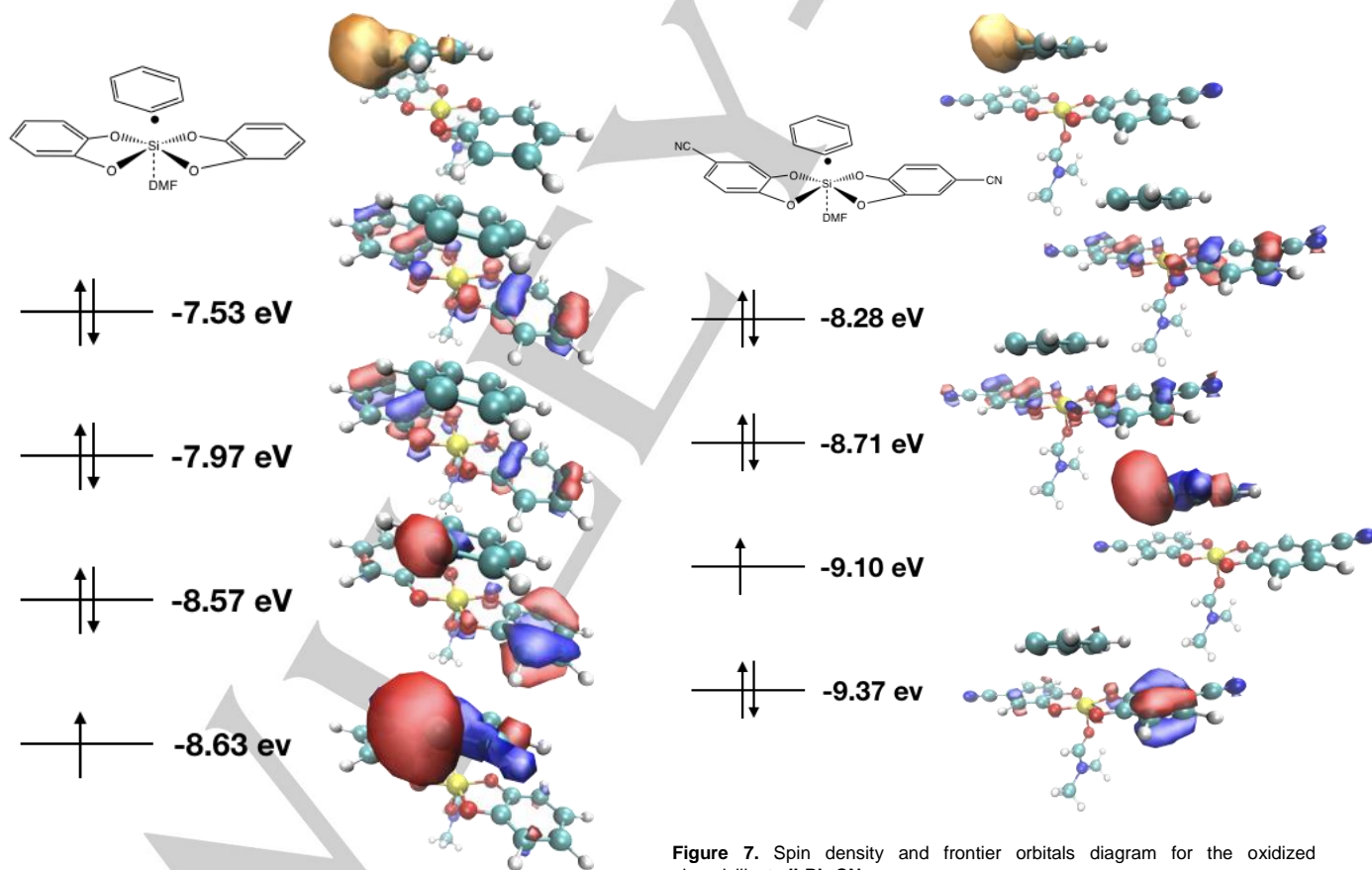
Figure 6. Spin density and frontier orbitals diagram for the oxidized aryl silicate II•Ph
