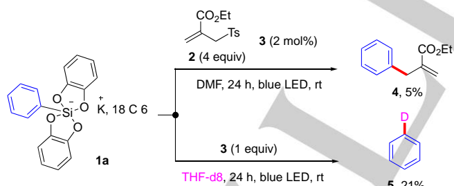
Scheme 3. Photooxidation of phenyl silicate 1a and phenyl radical trapping
