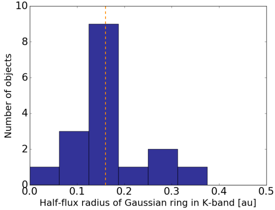
Fig. 3. Histogram of the half-flux radius of the ring model in the K band of our sample. The orange dashed line corresponds to the median value.
