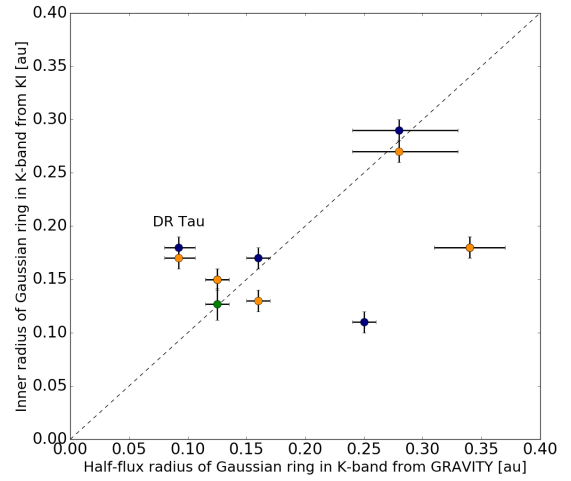
Fig. E.2. Inner radii of the ring in the K band derived from the KI by Eisner et al. (2010) (orange symbols), by Eisner et al. (2014) (blue symbols), and by Akeson et al. (2005) (green symbol) as a function of the half-flux radii in the K band derived from GRAVITY. The dashed line shows the 1:1 relation.
