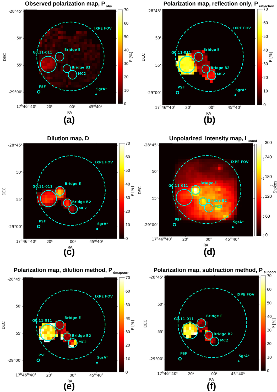
Fig. 7. Maps of the Sgr A complex IXPE FOV. (a) Observed polarization map. For clarity, we show the results for an average of 100 simulations. (b) Polarization map when only the MC reflection component is considered. (c) Dilution map. (d) Unpolarized intensity Stokes parameter map. (e) Reconstructed polarization map from dilution map method. (f) Reconstructed polarization map from subtraction method. The IXPE FOV and the cloud regions are displayed as in Fig. 5. For the maps (a), (b), (c), (e), and (f) the color-bar displays the polarization degree. For map (d) it displays the Stokes intensity parameter. The maps have a 30'' spatial binning and are obtained in the 4–8 keV energy band.
