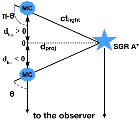
Fig. 1. Scattering geometry for a MC located in front or behind the Sgr A* plane. The two positions depicted have scattering angles \theta and \pi - \theta , which result in the same polarization degree. In addition, d_{\text{proj}} is the cloud-Sgr A* distance projected in the plane of the sky, d_{\text{los}} is the line-of-sight distance of the cloud with respect to the Sgr A* plane, c is the speed of light, and t_{\text{light}} is light travel time between Sgr A* and the cloud. The vector d_{\text{los}} assumes negative values if the cloud is in front of the Sgr A* plane and positive if behind.
