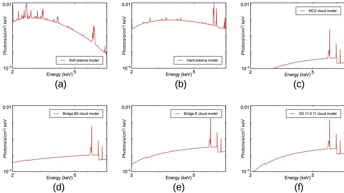
Fig. 4. Spectral models for the emission components of our simulations: the soft (a) and the hard (b) plasma in the nominal FOV, and the reflection in the MC2 (c), Bridge B2 (d), Bridge E (e), and G0.11-0.11 (f) region. The models were obtained from the Chandra spectral analysis performed in the present work and in Di Gesu et al. (2020) .
