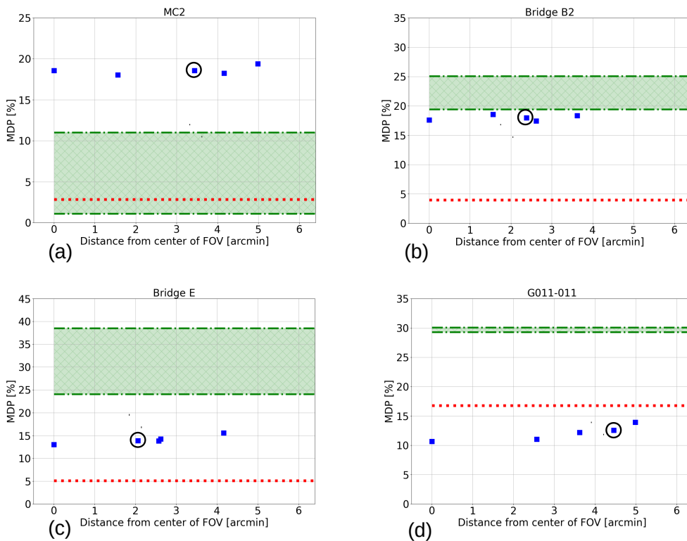
Fig. 6. MDP in the 4.0–8.0 keV band (square data points) for a 2 Ms-long observation as a function of the distance from the center of the FOV for the clouds MC2 (a), Bridge B2 (b), Bridge E (c), and G0.11-0.11 (d). The circled data points refer to the MC distance from the center of the FOV in the nominal IXPE pointing. The dashed line is the polarization degree from the model of Marin et al. (2015) diluted by the unpolarized emission in the 4–8 keV energy range. The shaded region within the dash-dotted lines covers the polarization degree range predicted for other line-of-sight distances for each MC reported in Table 1, diluted by the unpolarized emission in the 4–8 keV energy range.
