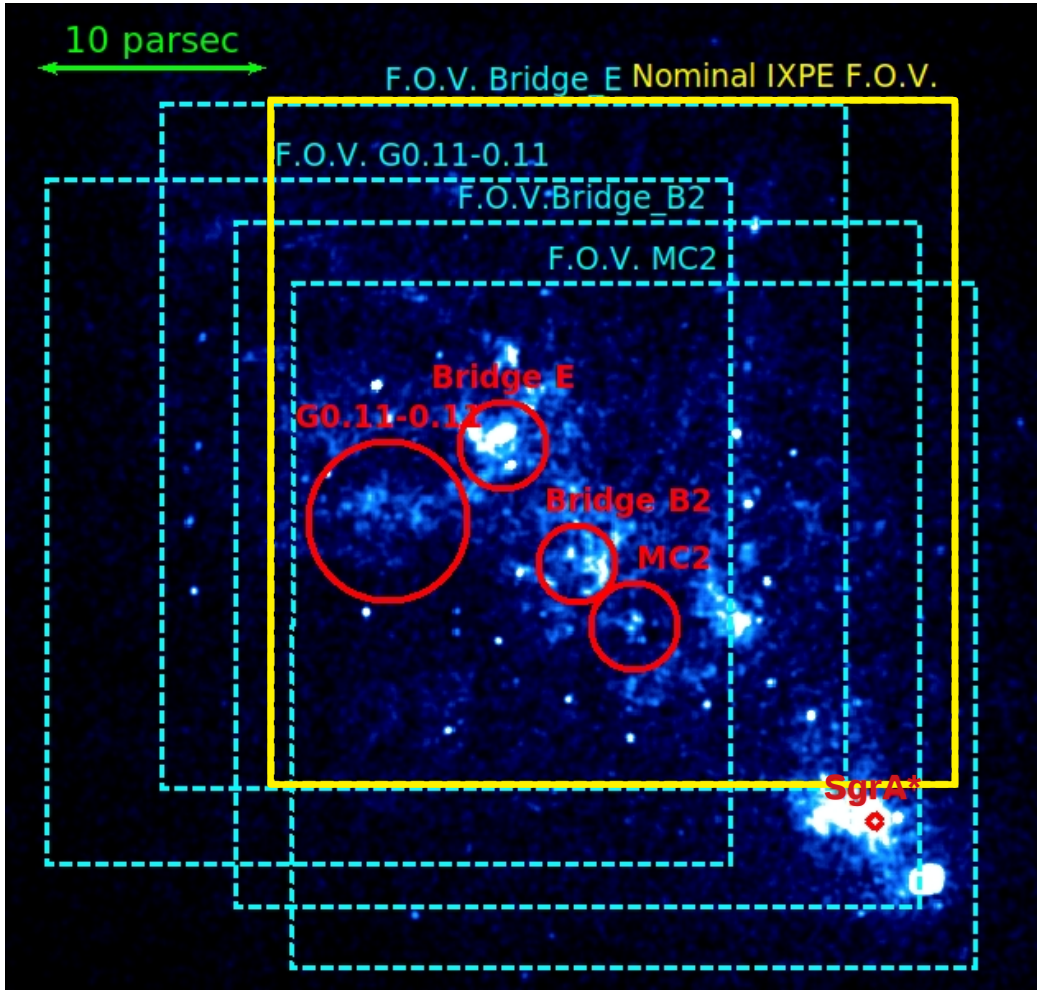
Fig. 2. Chandra Fe K \alpha map of the Sgr A complex. The dashed boxes are the FOVs considered in the analysis of Sect. 3.2, while the solid box represent the nominal IXPE FOV of our baseline simulation. The circles display the clouds considered in this work, while the diamond marks the position of Sgr A*. The double-headed arrow represents a distance of 10 pc.
