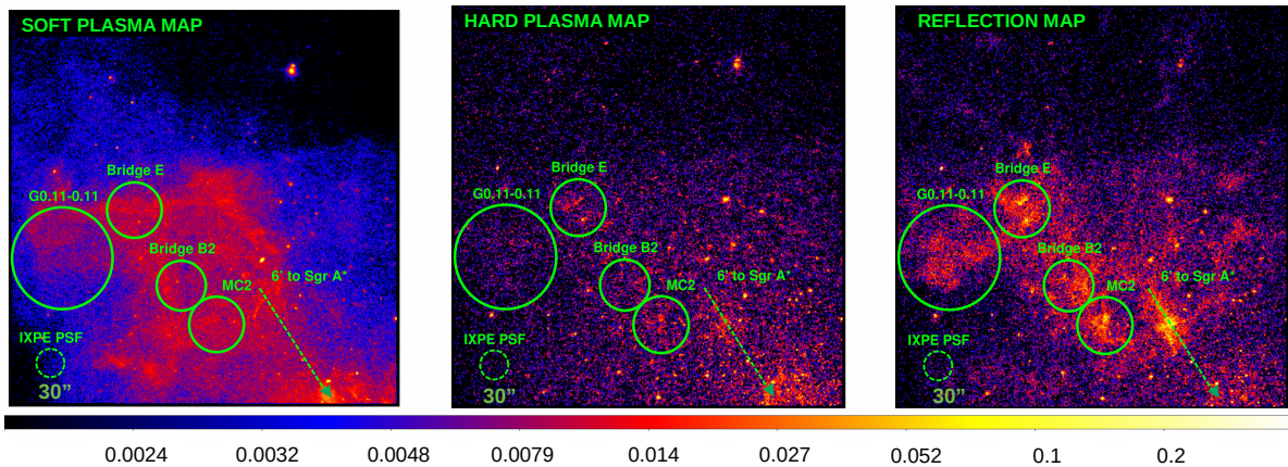
Fig. 3. Background- and continuum-subtracted, merged Chandra maps of the soft plasma, the hard plasma, and the reflection components in the Sgr A MC complex region centered on the nominal IXPE pointing (shown from left to right). The images are smoothed using a 3 pixel Gaussian kernel. The color bar displayed on the bottom has adimensional units because the images are normalized to the maximum value. The regions shown in the solid circles are the MC considered for IXPE simulations (i.e., MC2, Bridge B2, Bridge E, and G0.11-0.11). A dashed circle having the size of the IXPE PSF is shown for comparison. The direction to Sgr A* is indicated with a dashed arrow.
