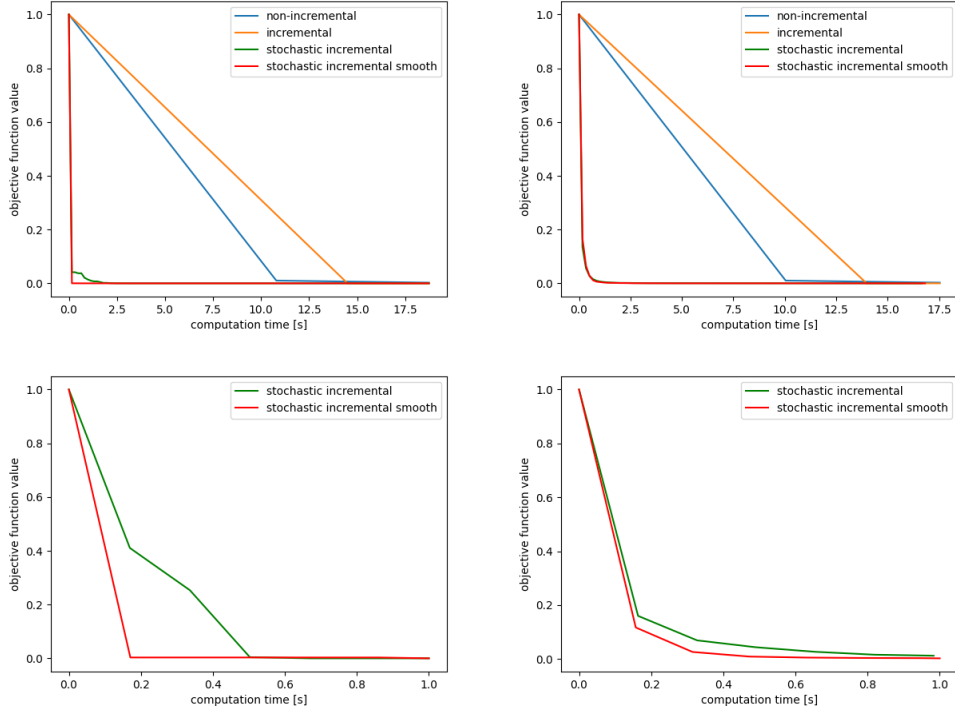
Figure 2: The plots show (f_N - f(x_{\text{best}}))/(f(x_0) - f(x_{\text{best}})) , where f_N := \min_{0 \leq k \leq N} f(x_k) , as a function of time, so x_k is the last iterate before a given point in time. In the first row we see the results after 17.5 seconds for one run left and 100 runs right. In the second row we see the results after 1 second for one run left and 100 runs right.
