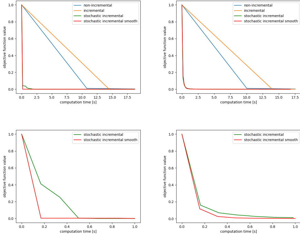
Figure 2: The plots show (f_N - f(x_{\text{best}})) / (f(x_0) - f(x_{\text{best}})) , where f_N := \min_{0 \leq k \leq N} f(x_k) , as a function of time, so x_k is the last iterate before a given point in time. In the first row we see the results after 17.5 seconds for one run left and 100 runs right. In the second row we see the results after 1 second for one run left and 100 runs right.
