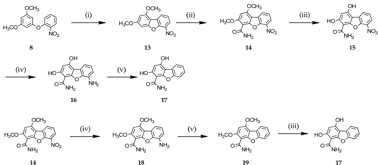
Scheme 2. Reagents and conditions: (i) \text{Pd}(\text{OAc})_2 , \text{AcOAg} , \text{PivOH} , 130\text{ }^\circ\text{C} , 4 h, 72%; (ii) \text{CSI} , \text{CH}_3\text{CN} , rt, 12 h, then \text{HCl} 5M, rt, 6 h, 53%; (iii) \text{Pyridine.HCl} , 200\text{ }^\circ\text{C} , MW, 15 min, 51% (for 15 ) and 48% (for 17 ); (iv) \text{Zn} dust, \text{NH}_4\text{Cl} , \text{CH}_3\text{OH} , 80\text{ }^\circ\text{C} , 2 h, 62% (for 16 ) and 49% (for 18 ); (v) \text{NaNO}_2 , \text{H}_2\text{SO}_4 , \text{EtOH} , 0\text{ }^\circ\text{C} , 30 min, then 80\text{ }^\circ\text{C} , 45 min, 52% (for 17 ) and 46% (for 19 ).
