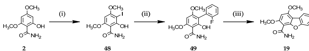
Scheme 5. Reagents and conditions: (i) NIS, CH 2 Cl 2 , 0 °C, 10 min, 60%; (ii) 2-Fluorophenylboronic acid, Pd(OAc) 2 , PPh 3 , K 3 PO 4 , CH 3 CN/H 2 O (4/1) sealed tube, 90 °C, MW, 2 h, 26%; (iii) Cs 2 CO 3 , CH 3 CN, 150 °C, MW, 1 h, 61%.
