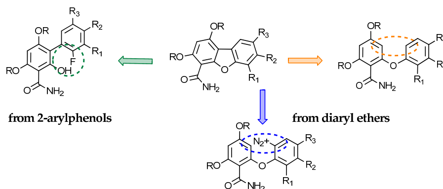
Figure 2. Proposed synthetic strategies to obtain the dibenzo[ b,d ]furan derivatives.
