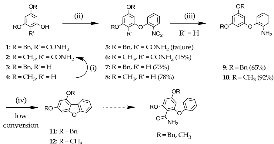
Scheme 1. Reagents and conditions: (i) CSI, CH 3 CN, 0 °C, 10 min, then HCl 5M, rt, 10 h, 45% (ii) KOH, DMF, 120 °C, 30 min, then 1-iodo-2-nitrobenzene, Cu(0), 170 °C, 24 h (for 5 and 6) and 2 h (for 7 and 8); (iii) Zn dust, NH 4 Cl, CH 3 OH, 80 °C, 2 h; (iv) (1) NaNO 2 , H 2 SO 4 , 0 °C, 45 min, (2) Cu(0), H 2 SO 4 , 60 °C, 24 h, 6% (for 11) and 11% (for 12) of conversion rates or Pd(OAc) 2 , EtOH, 60 °C, 24 h, 8% (for 11), and 28% (for 12) of conversion rates.
