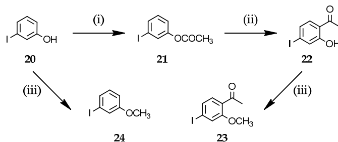
Scheme 3. Reagents and conditions: (i) \text{Ac}_2\text{O} , Pyridine, 130\text{ }^\circ\text{C} , 2 h, 90%; (ii) \text{BF}_3 \cdot 2\text{CH}_3\text{COOH} , 180\text{ }^\circ\text{C} , 12 h, 88%; (iii) \text{CH}_3\text{I} , \text{Cs}_2\text{CO}_3 , \text{CH}_3\text{CN} , 70\text{ }^\circ\text{C} , 2 h, 91% (for 23 ) and 4 h, 89% (for 24 ).
