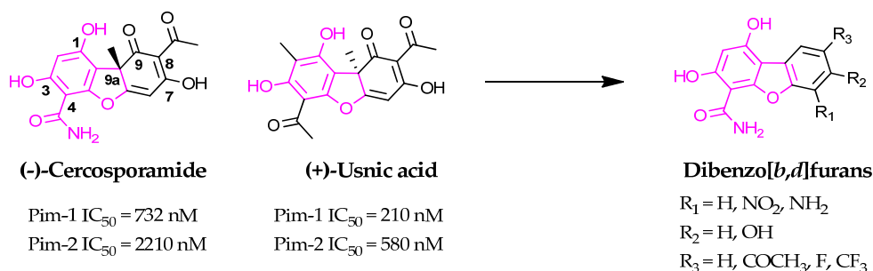
Figure 1. Drug design of the 1,3-dihydroxydibenzo[ b,d ]furan-4-carboxamide scaffold-based derivatives.
