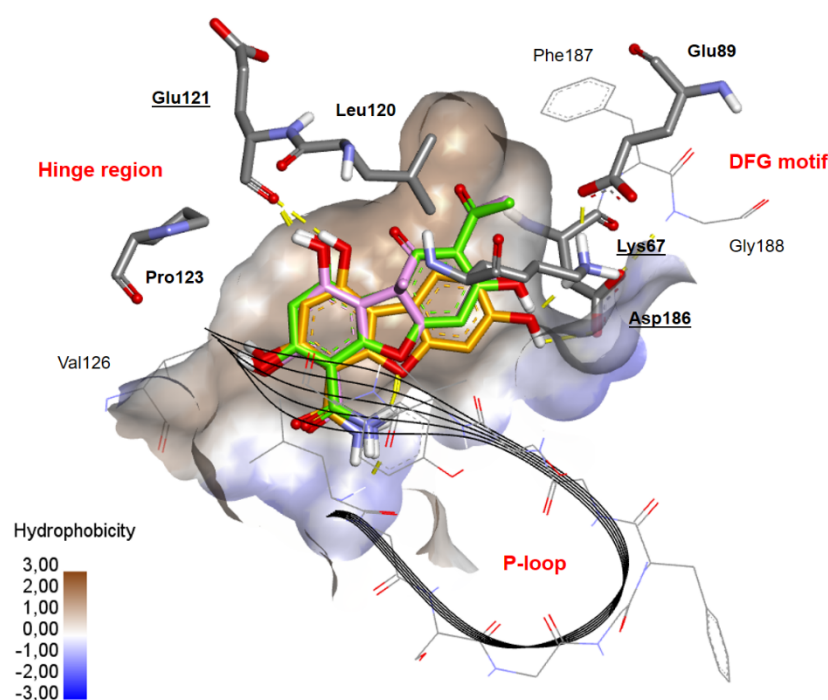
Figure 3. Binding pose found by the docking program GOLD for compound 44 (orange), compound 43 (green), and cercosporamide (pink) within the ATP pocket of Pim-1 (PDB ID 3A99). Hydrogen bonds are indicated as yellow lines.
