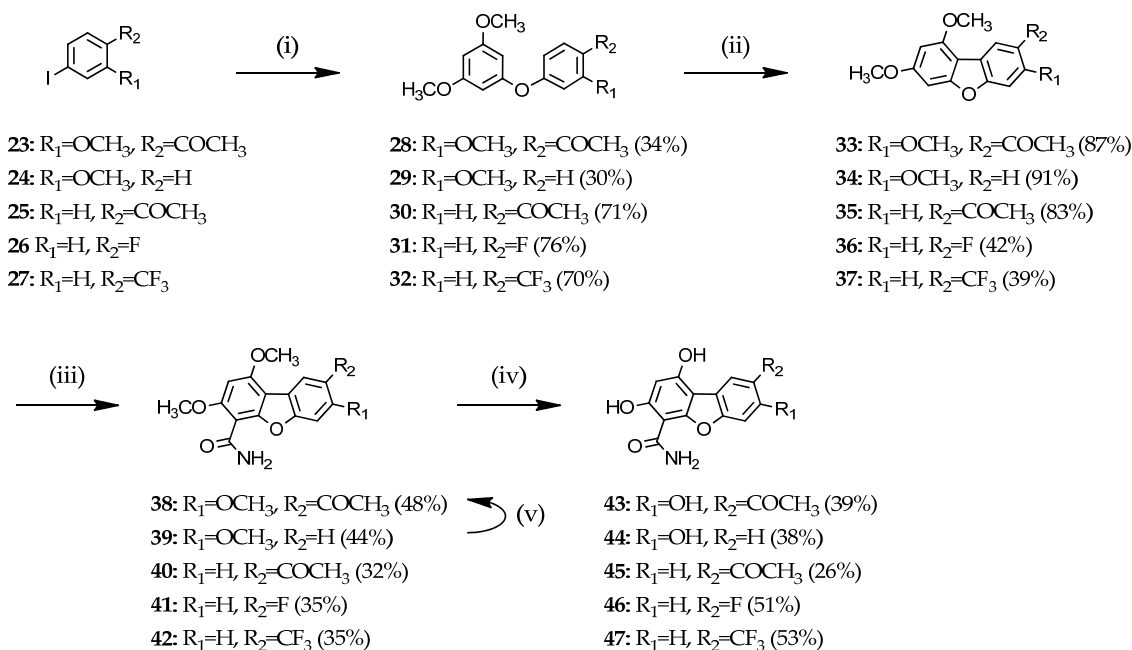
Scheme 4. Reagents and conditions: (i) 3,5-Dimethoxyphenol 4 , \text{Cs}_2\text{CO}_3 , \text{CuI} , \text{DMF} , 110\text{ }^\circ\text{C} , MW, 1 h; (ii) \text{Pd}(\text{OAc})_2 , \text{AgOAc} , \text{PivOH} , 130\text{ }^\circ\text{C} , 4–24 h; (iii) \text{CSI} , \text{CH}_3\text{CN} , 0\text{ }^\circ\text{C} –rt, 6–12 h, then \text{HCl} 5M, rt, 6–12 h; (iv) \text{Pyridine.HCl} , 200\text{ }^\circ\text{C} , MW, 15 min; (v) \text{AcCl} , \text{AlCl}_3 , \text{Cl-CH}_2\text{CH}_2\text{Cl} , rt, 1 h, 74%.
