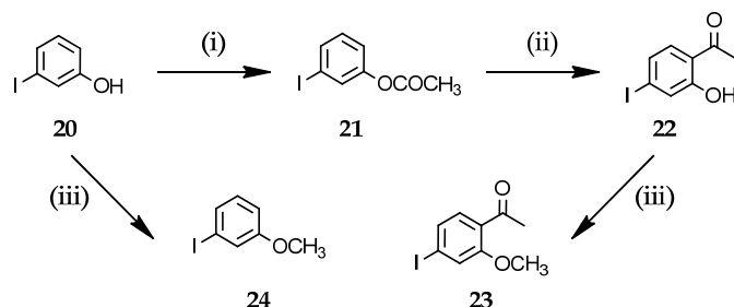
Scheme 3. Reagents and conditions: (i) \text{Ac}_2\text{O} , Pyridine, 130^\circ\text{C} , 2 h, 90%; (ii) \text{BF}_3 \cdot 2\text{CH}_3\text{COOH} , 180^\circ\text{C} , 12 h, 88%; (iii) \text{CH}_3\text{I} , \text{Cs}_2\text{CO}_3 , \text{CH}_3\text{CN} , 70^\circ\text{C} , 2 h, 91% (for 23 ) and 4 h, 89% (for 24 ).
