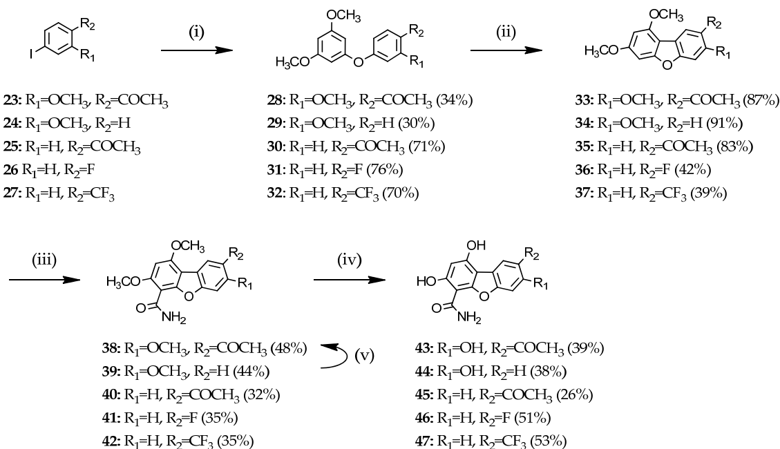
Scheme 4. Reagents and conditions: (i) 3,5-Dimethoxyphenol 4 , \text{Cs}_2\text{CO}_3 , \text{CuI} , \text{DMF} , 110^\circ\text{C} , MW, 1 h; (ii) \text{Pd}(\text{OAc})_2 , \text{AgOAc} , \text{PivOH} , 130^\circ\text{C} , 4–24 h; (iii) \text{CSi} , \text{CH}_3\text{CN} , 0^\circ\text{C} –rt, 6–12 h, then \text{HCl} 5M, rt, 6–12 h; (iv) \text{Pyridine} \cdot \text{HCl} , 200^\circ\text{C} , MW, 15 min; (v) \text{AcCl} , \text{AlCl}_3 , \text{Cl-CH}_2\text{CH}_2\text{Cl} , rt, 1 h, 74%.
