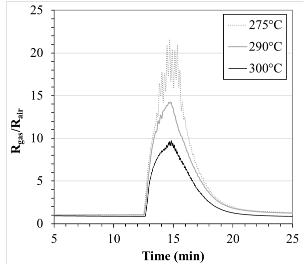
Fig. 6. Normalized responses for 5 000 ppm of CO 2 at 50%R.H for sensors fabricated by screen printe. (parameters: 1V/10μA/500 SCCM).
