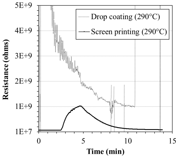
Fig. 5. Resistance variation to CO 2 exposure at 290°C in 50% humidity for La 2 O 2 CO 3 films obtained by drop coating and screen printing.
