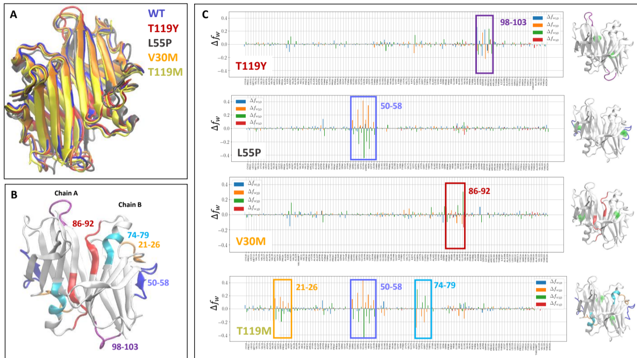
Fig. 2. Transthyretin (TTR) variants. A: Superposition of the X-ray structures of the TTR dimer variants: WT (PDB: 1f41), T119Y (PDB: 4tne), L55P (PDB: 3djz), V30M (PDB: 3kgs) and T119M (PDB: 1bze). B: X-ray structure of the WT TTR dimer. The segments involved in changes in local structural-level allocation in the variants with respect to the WT are highlighted. C: Changes in the local structural-level allocation of atomic interactions in the TTR variants compared to WT TTR (chain A), where \Delta f_{w_{1D},i} = f_{w_{1D},i}^{variant} - f_{w_{1D},i}^{WT} (and similarly for \Delta f_{w_{2D},i} , \Delta f_{w_{3D},i} and \Delta f_{w_{4D},i} ). Positive (negative) values of \Delta f_{w_{x},i} mean that residue i allocates a higher (lower) fraction of contacts to the x structural level in the variant compared to the WT. Next to each plot, the segment involved in changes in local structural-level allocation of atomic interactions in the variants compared to the WT TTR are highlighted in the variant's X-ray structure, with the same color code as the boxes in the plots and panel B. The mutated position is highlighted in green.
