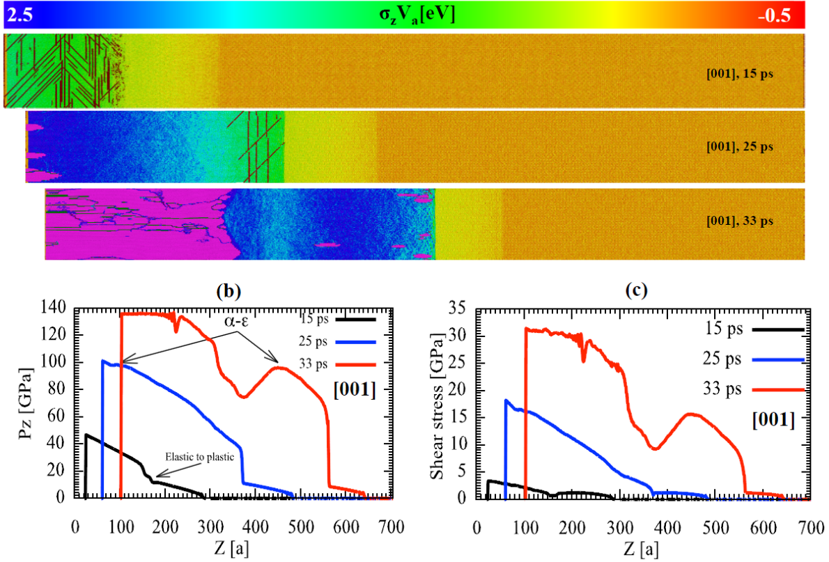
FIGURE 2: (a) Atomic structure snapshots at 15, 25 and 33 ps simulation times for [001]-oriented defect-free single crystal iron ramp-compressed to piston maximum velocity of 1600 m.s -1 (corresponding to maximum P_z of about 140 GPa) within 30 ps. Atoms color codes are the same as in Fig. 1 (a). Corresponding profiles of longitudinal pressure P_z (b) and shear stress (c).
