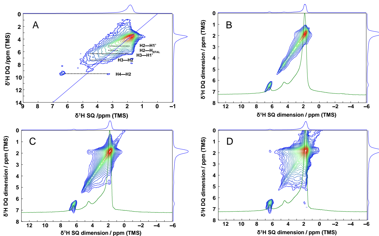
Figure 4. (A) 1\text{H}-1\text{H} SQ-DQ BABA spectrum of USY zeolite dried at 200^\circ\text{C} for 12 h. The dotted horizontal lines highlight a correlation, verified by the extraction of corresponding slices of the direct dimension. 1\text{H}-1\text{H} magnetization exchange spectra of USY zeolite dried at 200^\circ\text{C} for 12 h, with mixing times of (B) 5 ms, (C) 50 ms, and (D) 500 ms.
