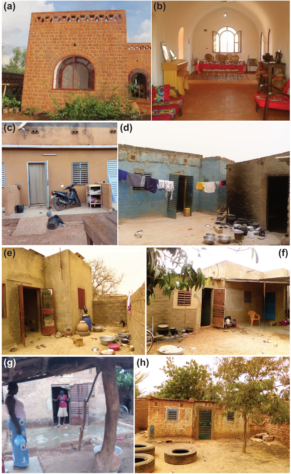
185 Figure 2 Pictures of the seven houses. (a–b) Somgandé Nubian Vault; (c) Kilwin Cement; (d) Nonghin Banco; (e) Nioko Cement; (f) Nioko Banco; (g) Polesgo Cement; (h) Polesgo Banco. See main text and Table 1 for details.
