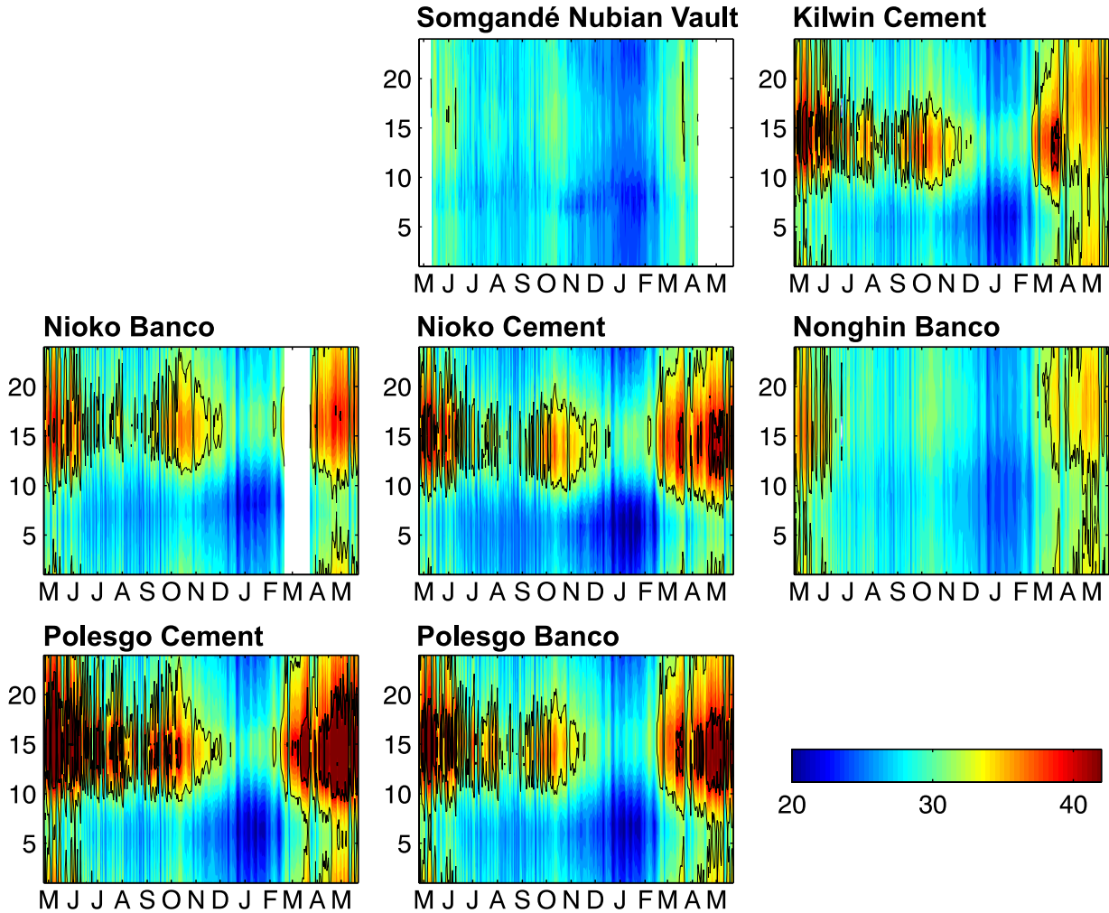
600 Figure 10 Daily vs. hourly diagrams of indoor heat index for the recording period between 25 April 2017 and 22 May 2018. Thin black contours show the “Extreme Caution” threshold. Thick black contours show the “Danger” threshold.
