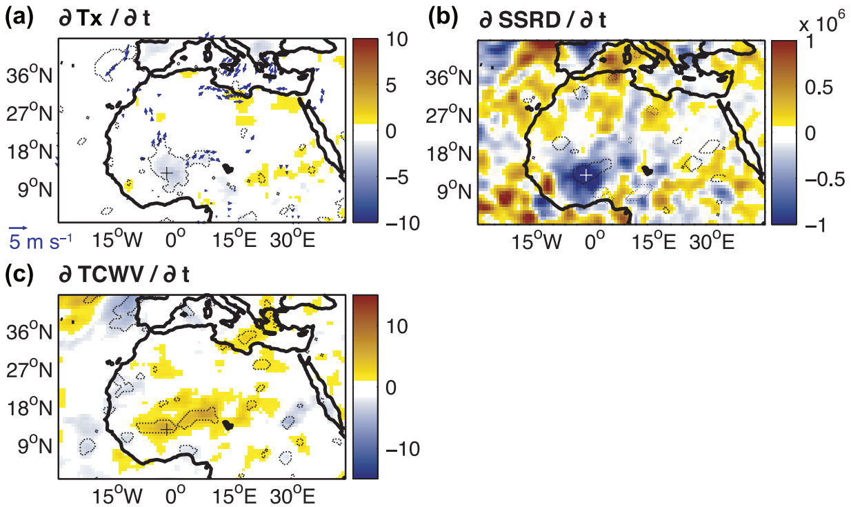
Figure 8 Abrupt decrease in Tx outdoor air temperature, and associated regional-scale mechanisms. (a) Changes in maximum air temperature at 2 m above ground level (Tx, in °C) and horizontal wind ( \text{m}\cdot\text{s}^{-1} ) at 10 m between the day before and the day of the abrupt decrease in Tx ( d_1 minus d_0 ). Dashed curves show statistically significant changes according to a t-test at the 95% confidence level. All fields are from ERA-Interim reanalysis. The plus sign shows the location of Ouagadougou. (b) As (a) but for downward solar radiation at the surface at 15:00 UTC ( \text{J}\cdot\text{m}^{-2} ). (c) As (a) but for total water vapour integrated vertically on the air column at 15:00 UTC ( \text{g}\cdot\text{m}^{-2} ).
