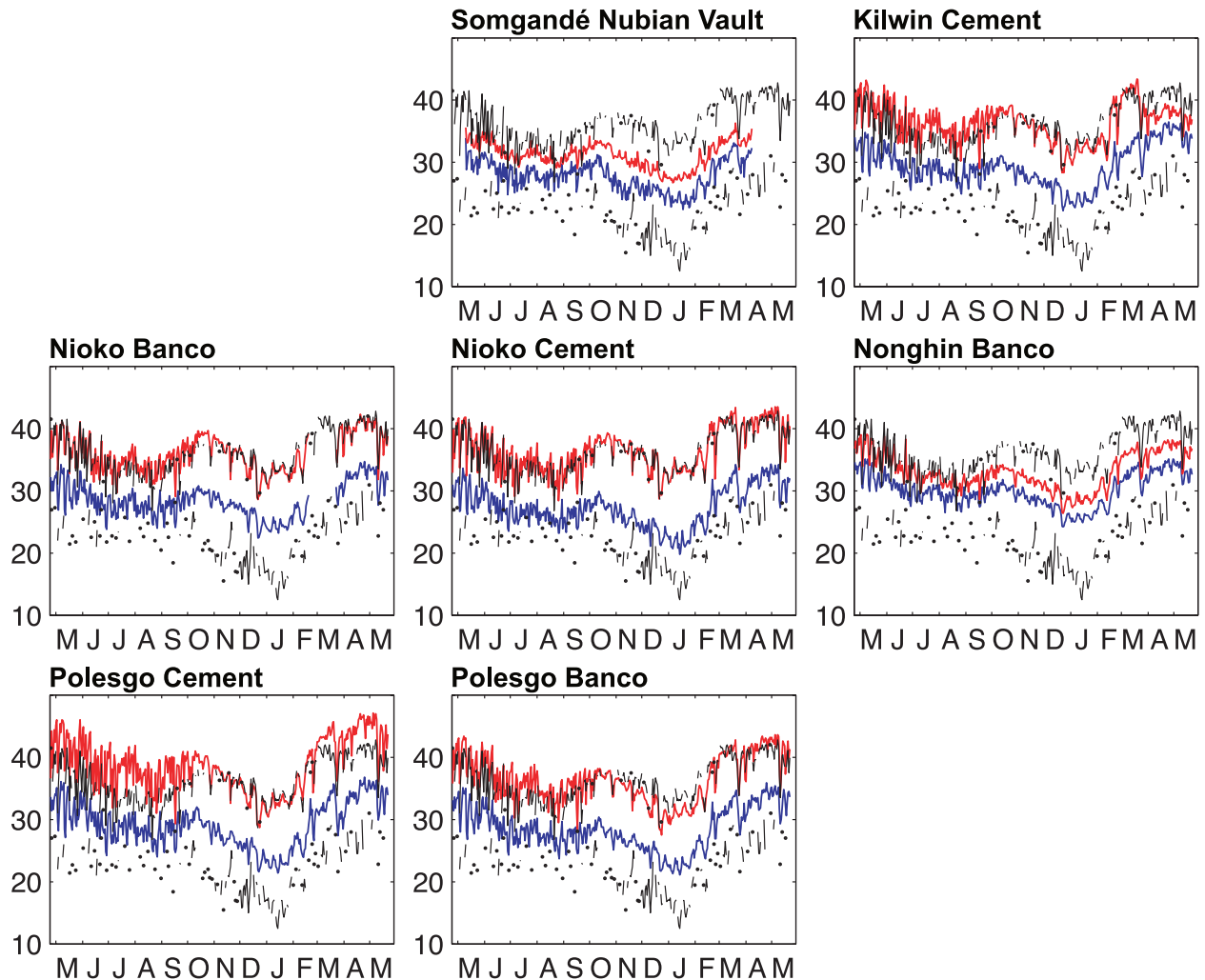
395 Figure 5 Daily minimum and maximum temperature at the synoptic weather station of Ouagadougou (black curves) and minimum (blue curves) and maximum (red curves) indoor temperature in each individual house.
