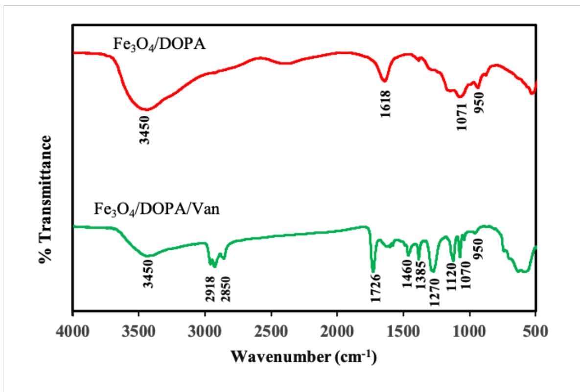
Fig. 5 FTIR spectra of (a) dopamine coated \text{Fe}_3\text{O}_4 NPs after oleic acid replacement by ligand exchange method and (b) Vancomycin conjugated magnetic \text{Fe}_3\text{O}_4/\text{DOPA}/\text{Van} nanoparticles.
