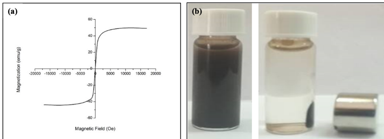
Fig. 4 (a) Magnetization value obtain from vibrating sample magnetometer (VSM) of \text{Fe}_3\text{O}_4 NPs as a function of magnetic field strength (Oersted) and (b) Digital photograph of oleic acid coated \text{Fe}_3\text{O}_4 NPs suspension in absence and presence of a magnetic field.
