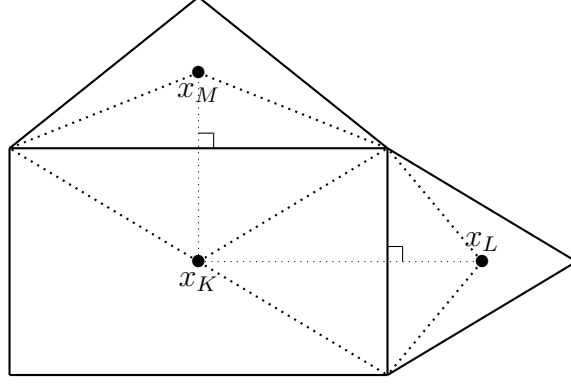
Figure 9: TPFA meshes
