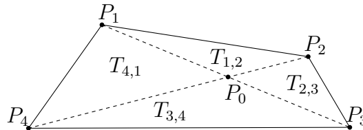
Figure 3: Case of a convex quadrangle K .
