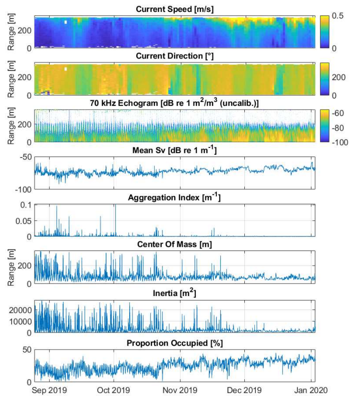
Fig. 12. Current speed, current direction and the monochromatic 70 kHz Echogram, plus key “Echometrics” from Echoview software. Mean Sv is a proxy for biomass, Aggregation Index is a measure of patchiness, Center of Mass shows the average depth of backscatter weighted by backscattering strength, Inertia is the spread of biomass from the center of mass, and Proportion Occupied is the percentage of the water column that contains backscatter.
