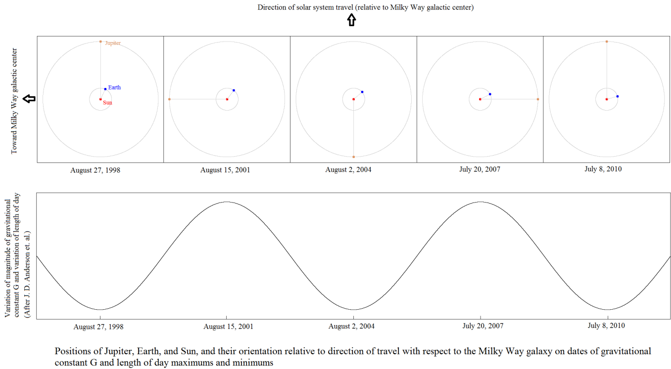
Figure 1. Correspondence between period and phase of varying G, LOD, and Jupiter's half orbital period
