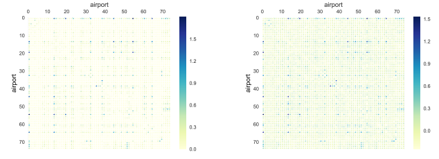
Fig. 8. Illustration of the graph-structured input of MSTAGCN and MSTAGCN-NA. The left matrix represents the scheduled structure of an airport network (MSTAGCN-NA). An example of the corresponding adaptive matrix learned by our model is represented in the right matrix (MSTAGCN).
