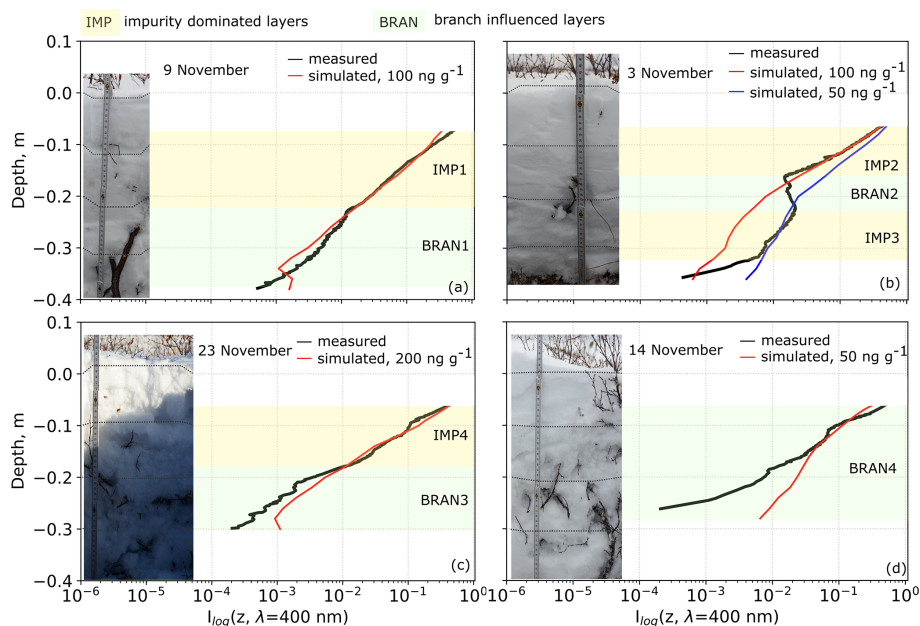
Figure 6. Log-irradiance and SnowMCMC simulations at 400 nm for measurements taken on (a) 9 November, (b) 3 November, (c) 23 November and (d) 14 November in snowpacks with shrubs. Yellow shaded areas highlight layers where measured log-irradiance profiles and SnowMCMC simulations fitted well. Green shaded areas highlight layers where log-irradiance and SnowMCMC simulations fit less well and branches were visible in the snowpit photographs.
