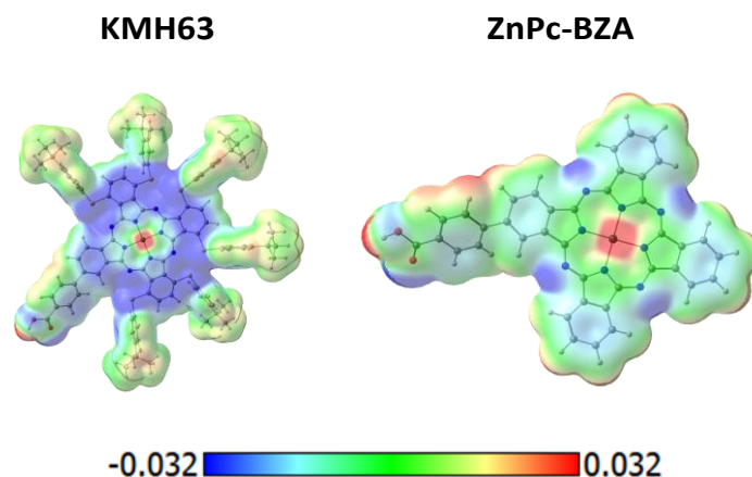
Figure 3. Molecular electrostatic potential calculated at the M06/6-31G(d,p) level of theory in dichloromethane. The color scale is added in bottom.
