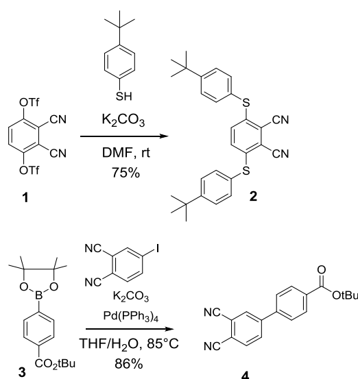
Scheme 1. Synthesis of phthalonitrile 2 and 4.
