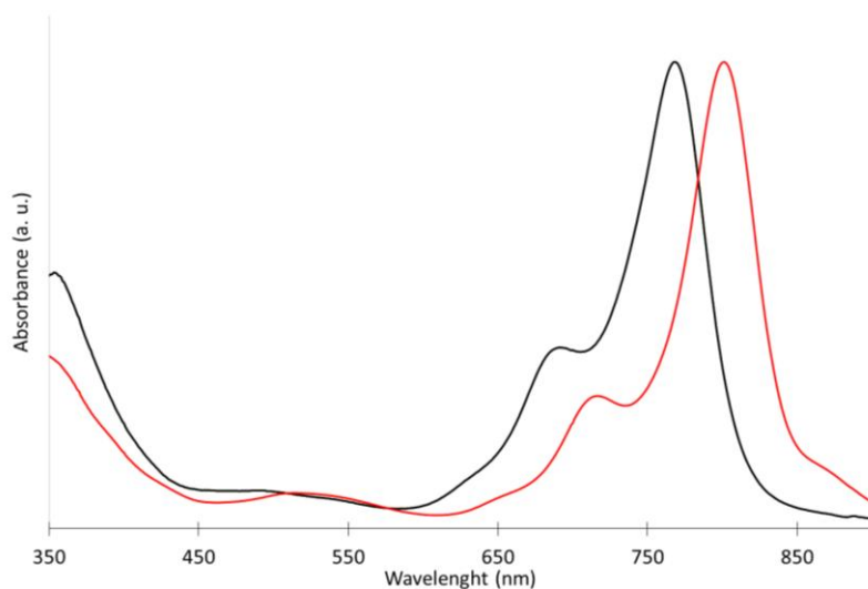
Figure 1. Normalized absorption of KMH63 (black) and Zn-Pc-1 (red) recorded in dichloromethane solution.
