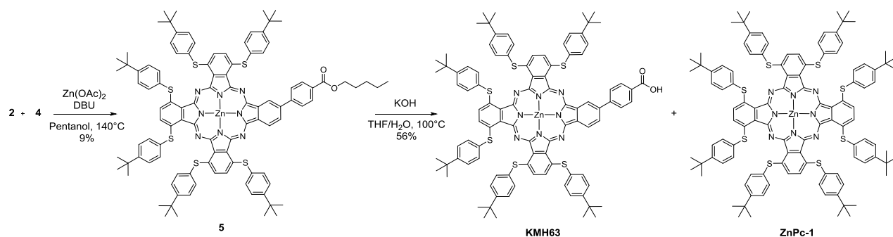
Scheme 2. Synthesis of zinc phthalocyanine KMH63 .
