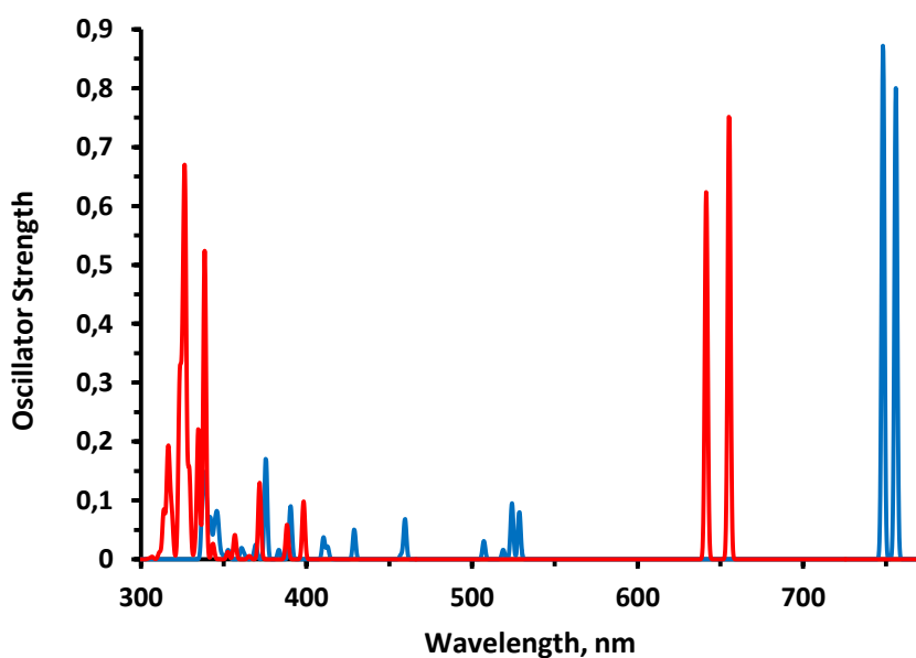
Figure 4. Electronic absorption spectra calculated at the M06/6-31G(d,p) level of theory in dichloromethane; KMH63 blue and ZnPc-BZA red.
