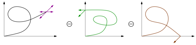
Figure 3: Functional equation for Gessel walks, pictorially.
