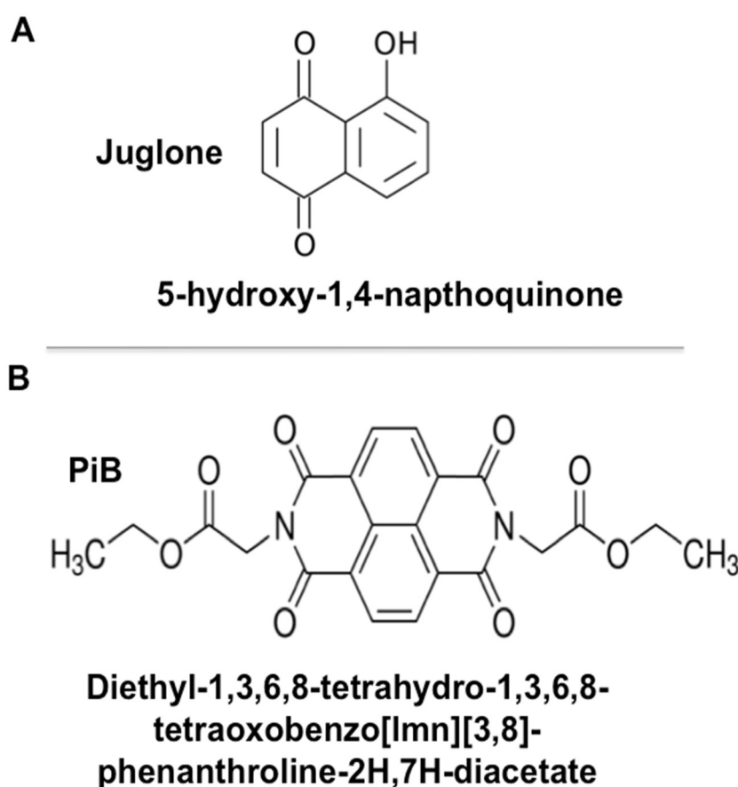
Figure 1. Molecular structure of juglone and PiB. (A) Juglone (5-hydroxy-1, 4-naphthoquinone) is a natural compound extracted from walnut leaf. (B) PiB (diethyl-1,3,6,8-tetrahydro-1,3,6,8-tetraoxobenzo[lmn]-phenanthroline-2,7-diacetate) is a chemical synthetic agent.
