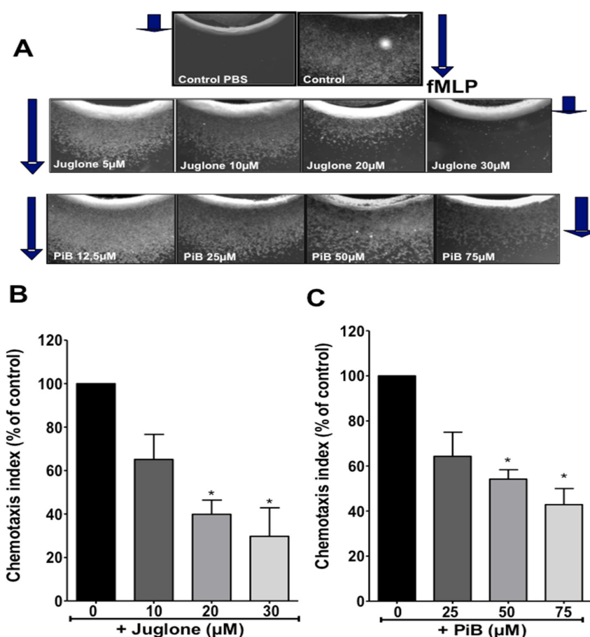
Figure 3. Effect of juglone and PiB on neutrophil chemotaxis. (A) Neutrophils ( 100 \times 10^6 cell/mL) were pretreated with increasing concentration of juglone (0, 10, 20, 30 \mu\text{M} ) or PiB (0, 25, 50, 75 \mu\text{M} ). Cells (5 \mu\text{L} ) are added to the agarose central well, 5 \mu\text{L} of the chemoattractant fMLP ( 10^{-7} M) or buffer PBS are placed in the other wells, the plates are incubated for 2 h at 37 ^{\circ}\text{C} . Results were observed using a ZEISS microscope. The direction of migration towards fMLP is shown by the arrows. (B,C) The chemotaxis index is determined as the distance of cell migration to fMLP. Results are represented as the ratio to fMLP without inhibitors (100%). Histograms represent the percentage of inhibition of cell migration, in the presence of Pin1 inhibitors. Data are means \pm S.E.M. of 4 separate experiments (* p < 0.01 ).
