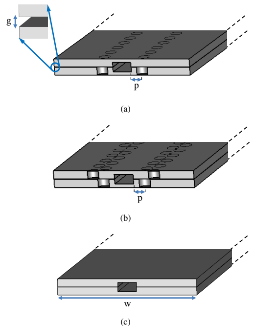
Fig. 4. RW made of two layers with an air gap in between: (a) One row of glide-symmetric holes at the location of gap. (b) Two rows of glide-symmetric holes at the location of gap. (c) No holey structure at the location of gap.
