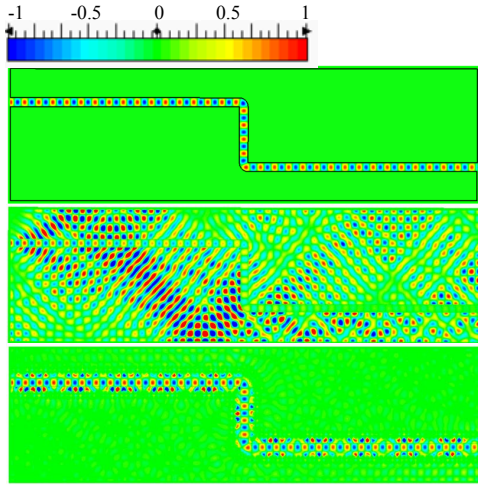
Fig. 8. Normalized electric field distribution of (a) a double 90° bent aluminum RW, (b) a waveguide with an air gap on the side walls, (c) the proposed waveguide structure with a glide-symmetric holey EBG.
