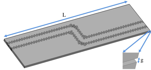
Fig. 6. Structure of a double 90° bent waveguide with two rows of glide-symmetric holey EBG at the location of the gap on side walls. ( L=25 cm)
