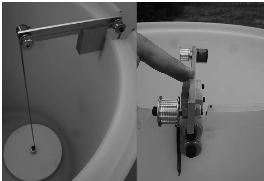
Fig. 2 - Floating level system.
