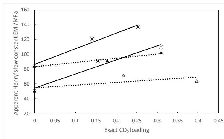
A B Figure 8: Variation of Methanethiol (o, A) and Ethanethiol (Δ, B) apparent Henry's law constant as a function CO 2 loading (H 2 S loading is fixed). Empty symbol: 333K, black symbol: 365 K. Lines: linear tendency curve. x: without H 2 S at 333K, *: with H 2 S at 365 K.
