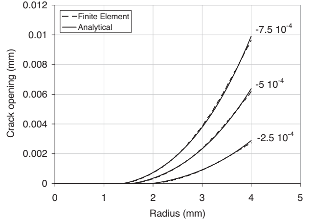
Fig. 4. Impact of the thermal strains magnitude ( \epsilon_3^{an} = -2.5 \times 10^{-4} , -5 \times 10^{-4} and -7.5 \times 10^{-4} \text{ mm}^{-2} ) on the crack opening calculated with the finite element and analytical models.
