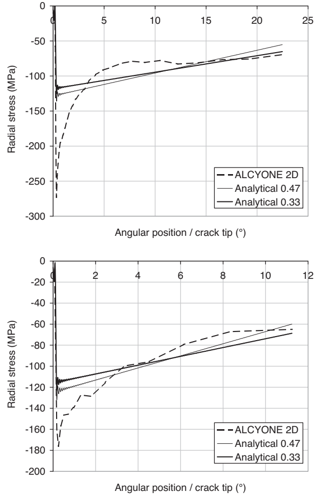
Fig. 17. Clad inner wall radial stress distribution as given by ALCYONE and the analytical models (top: N=8 , bottom: N=16 ).
