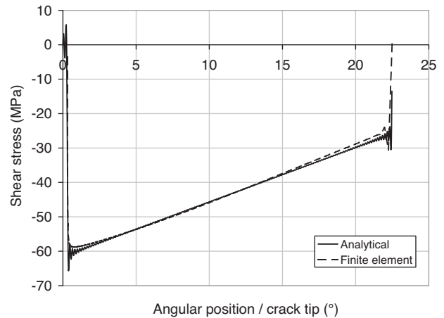
Fig. 10. Clad inner wall radial (top) and shear (bottom) stress distributions as given by the analytical and finite element models.
