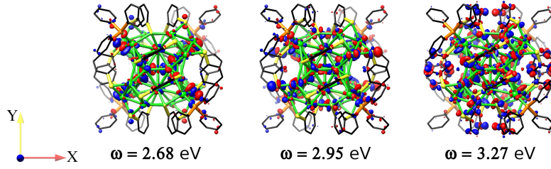
Fig. 4 Fourier-transformed induced densities in \text{Ag}_{29}(\text{BDT})_{12}(\text{TPP})_4 at energies (in the VIS) of 2.68, 2.95, and 3.27 eV are shown for an iso-surface value of \pm 2 \times 10^{-7} (red and blue), along with the atomic arrangements in the cluster. The perturbation was applied along the x axis. We show the reconstructed modes at a quarter period, details are explained in the Supplementary Material.
