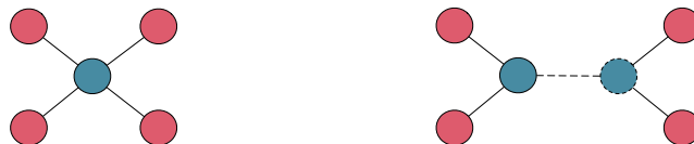
Figure 5: The 4-ary tree (on the left) can be transformed into an unrooted binary tree by adding a dummy vertex and a dummy edge (dashed, on the right).
