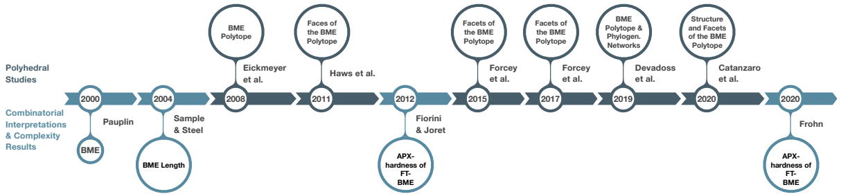
Figure 13: Graphical representation of the development of the BMEP's combinatorics, since Pauplin [121]'s article. The dark grey stages represent articles studying the polyhedral combinatorics of the BME polytope, including Eickmeyer et al. [46]'s conjectures, Haws et al. [71]'s faces, Forcey et al. [54]'s complete description of the BME polytope for n = 5 , Forcey et al. [55]'s further facets of the BME polytope and combinatorial connections with the permutoassociahedron, Devadoss et al. [42]'s connections of the BME polytope with split-networks, and Catanzaro et al. [28]'s recent advances. The blue stages represent articles presenting the combinatorial interpretation of the BME length function [144] as well as complexity results [52, 57].
