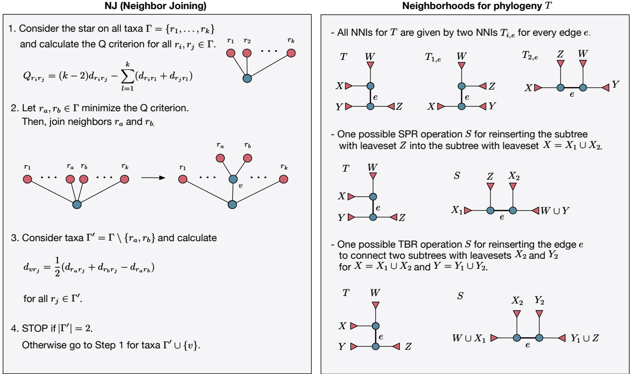
Figure 20: An example of two possible approximate approaches to solution of the BMEP. The figure on the left outlines the so called Neighbor Joining (NJ) method [65, 138, 151] i.e., a greedy constructive heuristic that starting from an infeasible solution to the problem (i.e., a star-tree) iteratively clusters two terminal leaves according to a specific optimality criterion, until a phylogeny of \Gamma is obtained. The figure on the right shows three examples of possible neighborhoods of a given phylogeny T . We can distinguish between the Nearest Neighbor Interchange (NNI), the Subtree Pruning and Regrafting (SPR), and the Tree Bisection and Reconnection (TBR), respectively [51, 60].
