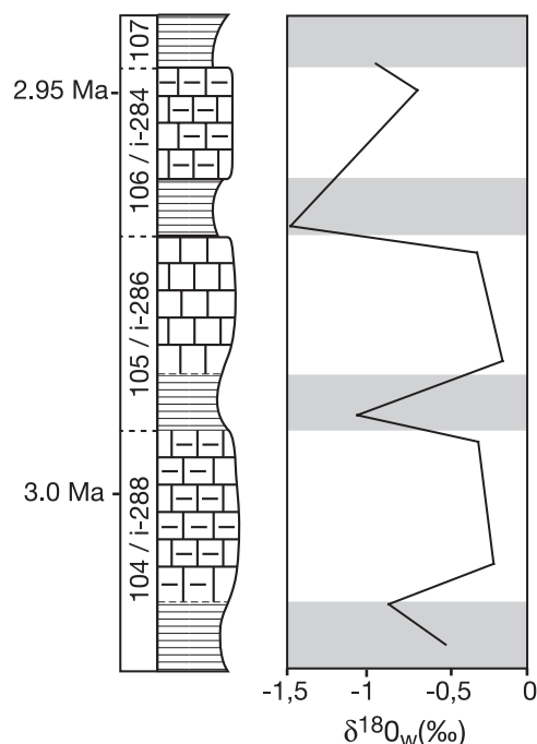
Figure 7. Evolution of seawater oxygen isotopic ratios ( \text{‰} SMOW) throughout the studied section.
