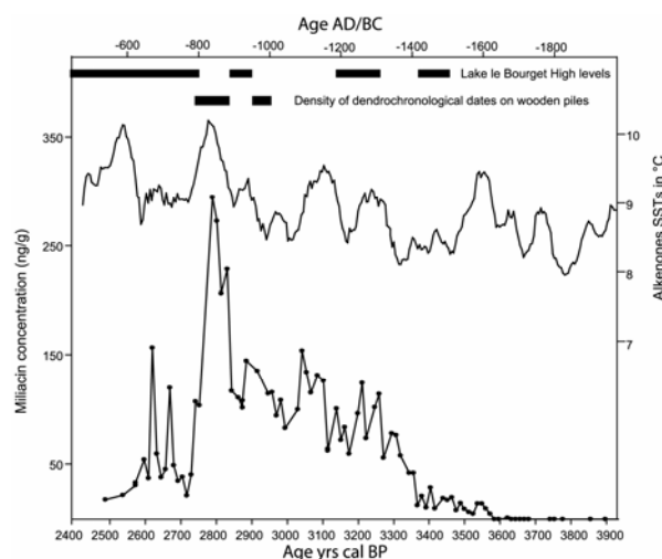
Fig. 1. Evolution of miliacin concentration, density of dendrochronological dates measured on wooden piles and periods of high lake levels for Lake le Bourget and alkenones-based SSTs reconstruction off Iceland for the 2000-600 BC time period.
