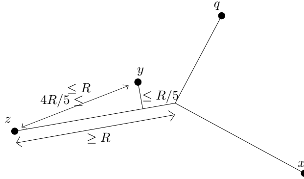
FIGURE 3. The geodesics from z to q and x follow-travel for at time at least R .
