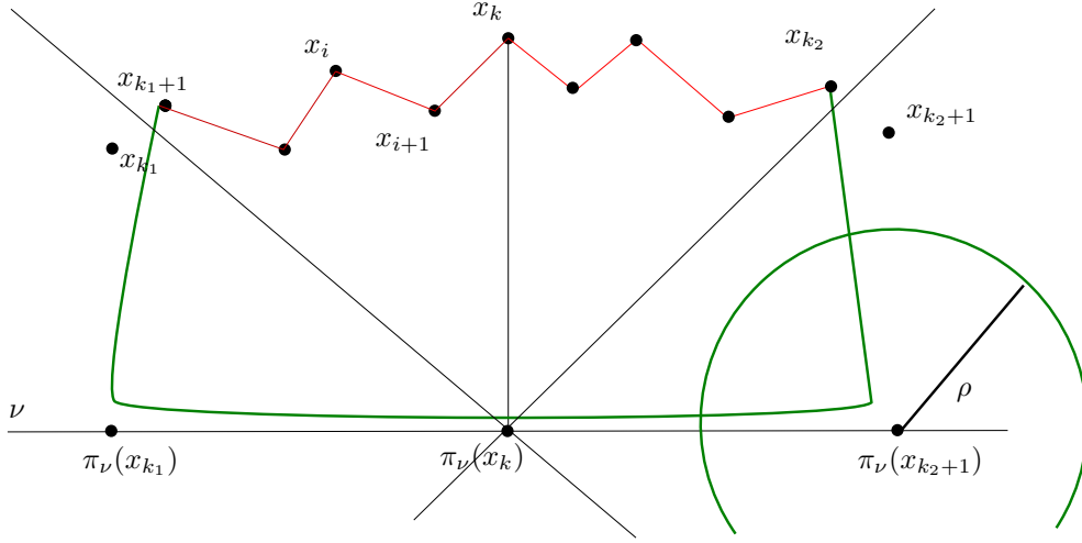
FIGURE 2. The green path represents the geodesic from x_{k_1+1} to x_{k_2} . Because of Items (2) and (3) of Lemma 8.4 their projections on v must remain close to those of x_{k_1} and x_{k_2+1} . From Item (1) and by construction of N_v(x_k) one of the distances d(\pi_v(x_{k_1}), \pi_v(x_k)) , d(\pi_v(x_{k_2+1}), \pi_v(x_k)) must be at least of the order \epsilon(k_2 - k_1)/5 . This prevents the red path to enter in at least one of the balls B(\pi_v(x_{k_1}), \rho) or B(\pi_v(x_{k_2+1}), \rho) , in green in the figure (with \rho = \epsilon(k_2 - k_1)/10 ). This implies that the length of the red path must be exponential in \rho since it avoids a ball through which the geodesic relating its endpoints passes (in green in the Figure).
