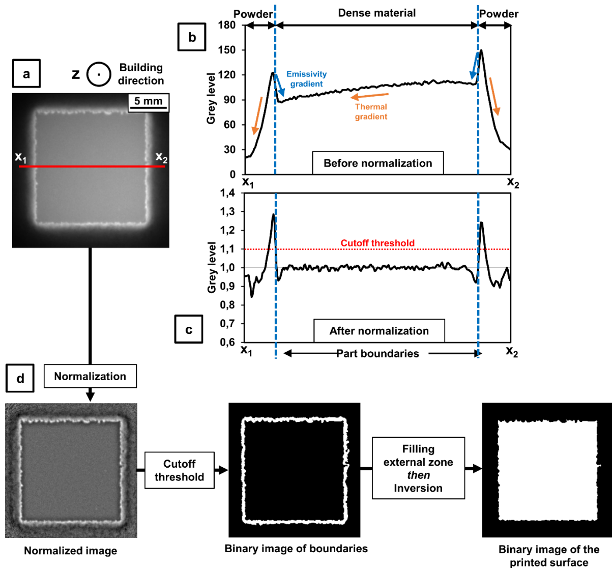
Fig. 4. Illustration of the part boundaries detection image processing routine. (a) NIR-image of a cube for which the grey level is plotted along the line defined by the two points x_1 and x_2 in (b). This grey level profile is affected by thermal gradients in the part, in the powder bed but also by the emissivity gradient between powder and dense material. The same grey level profile is plotted in (c) after NIR-image normalization subsequently to a background correction. Note that the background correction allows the thermal gradient to be removed but allows the emissivity gradient to be preserved. A final cutoff threshold can be applied to the corrected images to identify part boundaries. (d) Example showing the image processing steps to obtain a binary image of the printed surface.
