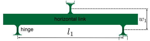
Fig. 6. Horizontal and vertical distances between hinges.
