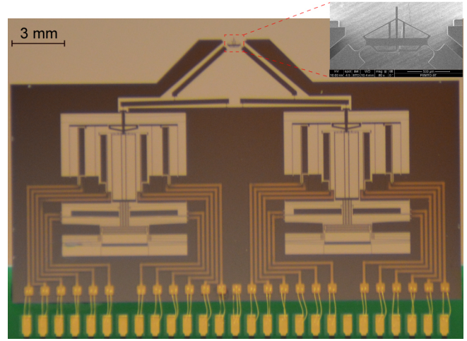
Fig. 10. Fabricated prototype.
