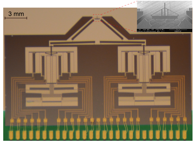
Fig. 10. Fabricated prototype.
