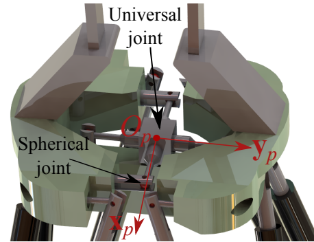
Fig. 5. Design of the configurable platform.
