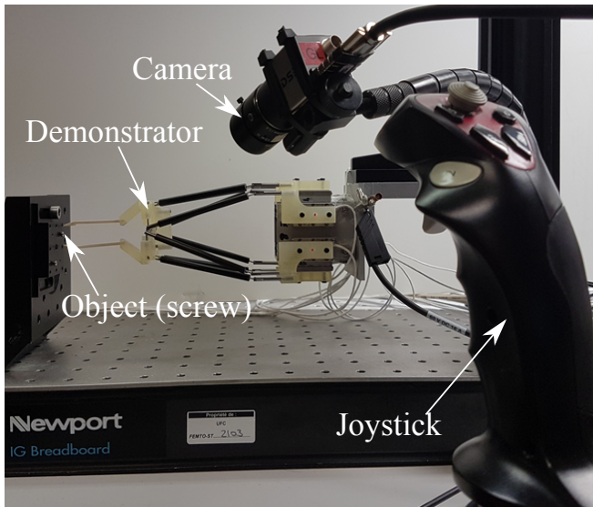
Fig. 6. Experimental setup.
