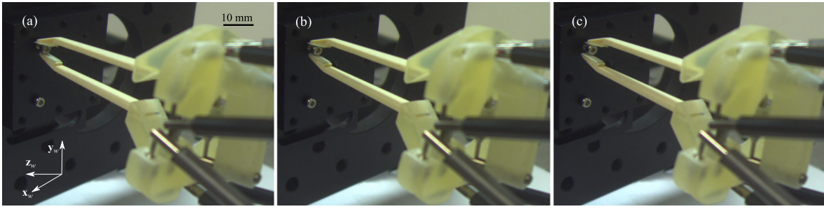
Fig. 7. Screwing a 2-mm screw using the twist mobility between the two fingers.
