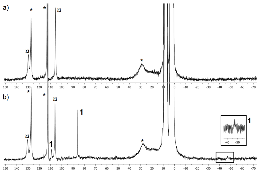
Figure 2: ^1\text{H} NMR spectra (60 MHz, 20 °C, \text{THF } d_8 ) of a) a 40:60 distribution of [\text{Mes}_2\text{Fe}^{\text{II}}\text{Br}]^- and [\text{Mes}_3\text{Fe}^{\text{II}}]^- (generated by addition of 10 equiv. [\text{nBu}_4\text{N}^+;\text{Br}^-] onto [\text{Mes}_4\text{Fe}_2^{\text{II}}] ) treated by 70 equiv. 2-PyCl at 20 °C during 4 h; and b) of a solution of [\text{Mes}_3\text{Fe}^{\text{II}}]^- (generated by addition of 4 equiv. \text{MesMgBr} onto \text{FeCl}_2 ) in the presence of an excess of 2-PyCl (70 equiv.), after addition of \text{PhMgBr} (2 equiv.); * = [\text{Mes}_3\text{Fe}^{\text{II}}]^- ; □ = [\text{Mes}_2\text{Fe}^{\text{II}}\text{Br}]^- .
