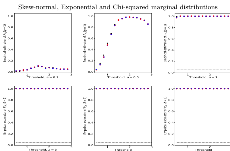
FIG 5. Under H_1 hypothesis. Average of the empirical values of \mathbb{P}_{H_1(t)}(\phi_m^P = 1) for different thresholds t , for 500 Montecarlo simulations for m = 512 with a skew-normal marginal distribution centered around its median value, with different choices of parameter a = 0.1, 0.5, 1, 3 (from first to fourth panel), Exp(1) - \theta distribution (fifth panel) and \chi^2 - \theta distribution of degree of freedom 1 (sixth panel), \theta been the median value of the image. We consider different test statistics: \phi_m^P(\hat{\sigma}^P) as in (12) (blue crosses), \phi_m^P(\hat{\sigma}^A) as in (13) (red diamonds) and \phi_m^{k-s}(\hat{\sigma}^{k-s}) as in (15) (black stars). Threshold \alpha = 0.05 is displayed by a dashed horizontal line.
