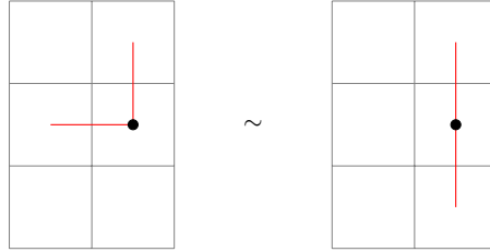
FIG 7. Representation of the configuration between (f_1(l, k), f_2(l+1, k-1)) (left panel) and (f_1(l, k), f_1(l, k+1)) (right panel), the black dot represents the cell (k, l) .
