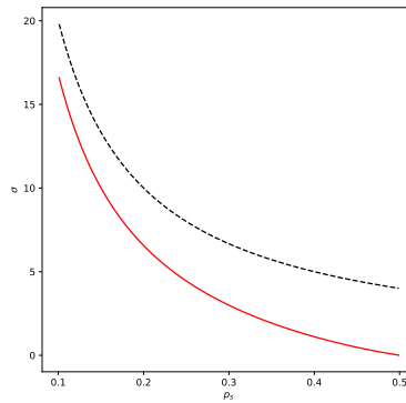
FIG 9. Variance values \sigma^2(s) in (7) in (red full line) and (\sigma_{k-s})^2(s) in (14) (black dashed line), for p_s \in (0.1, 0.5)
