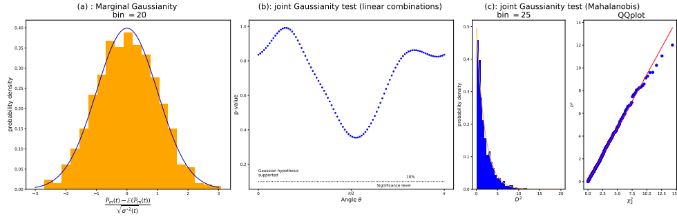
FIG 8. (a.) Univariate Gaussianity of A_m(t) in (26) for m = 1200 and t = 0.5 for a bin size equal to 20. The solid blue line represents the corresponding standard Gaussian density. We propose two validation methods of the multivariate Gaussianity of the bivariate vector (A_m(s), A_m(t)) with s = 0.6 and t = 0.2 . (b.) p -value for \cos(\theta)A_m(t) + \sin(\theta)A_m(s) for \theta \in [0, 2\pi) , computed using the function stats.normaltest from scipy . (c.) Estimated probability density of D^2 (blue histogram) and theoretical Chi-squared density (red curve). QQ-plot between the theoretically predicted \chi^2_2 quantiles and the empirical quantiles of D^2 .
