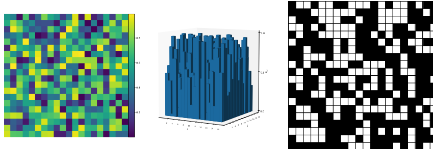
FIG 2. Left and center panels: Image of size (20 \times 20) realization of a Uniform white noise model. Right panel: Obtained binary image for t = 0.5 .
