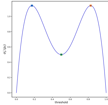
FIG 10. Curve of the variance function in Equation (4) for a Uniform white noise model for m = 1024 , the extrema are reached at p_t \in \{0.172, 0.5, 0.82\} .
