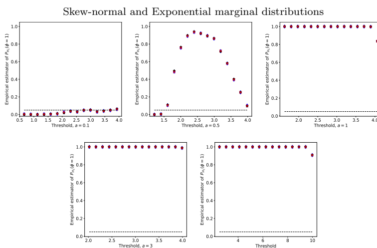
FIG 5. Under H_1 hypothesis. Average of the empirical values of \mathbb{P}_{H_1(t)}(\phi_m^{\mathcal{P}} = 1) for different thresholds t , for 500 Montecarlo simulations for m = 512 with a skew-normal marginal distribution with different choices of parameter a = 0.1, 0.5, 1, 3 (from first to fourth panel) and Exp(1) distribution (fifth panel). We consider different test statistics: \phi_m^{\mathcal{P}}(\hat{\sigma}^{\mathcal{P}}) as in (12) (blue diamonds), \phi_m^{\mathcal{P}}(\hat{\sigma}^{\mathcal{A}}) as in (13) (red crosses) and \phi_m^{k-s}(\hat{\sigma}^{k-s}) as in (15) (black stars).
