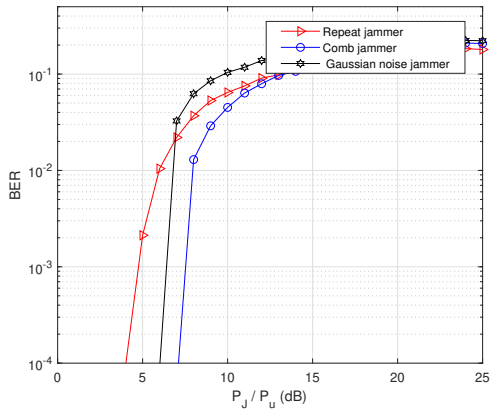
Fig. 7. BER comparison between the repeat jammer, the comb jammer and the Gaussian noise jammer in the first scenario and for the conventional BPSK constellation.
