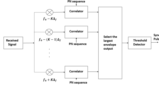
Fig. 2. Frame Synchronization and Initial search for Doppler frequency offset.
