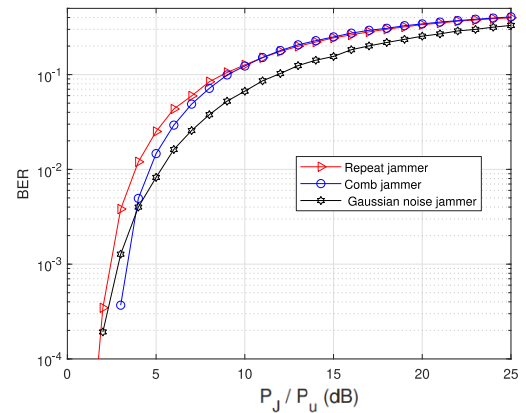
Fig. 12. BER comparison between the repeat jammer, the comb jammer and the Gaussian noise jammer in the second scenario, for the rotated UP-RCQD QPSK constellation and SF = 4 .
