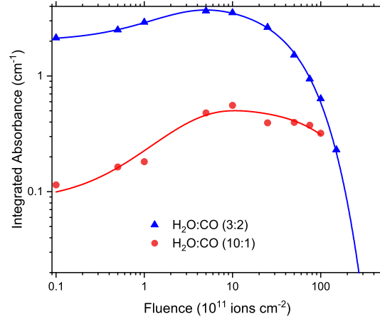
Figure 8. 2141 \text{cm}^{-1} component integrated absorbance as a function of fluence. Data are fitted by Eq. 1.
