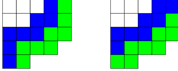
Figure 3: The 8-core of \lambda = (5, 5, 5, 4, 2) is \bar{\lambda} = (3, 2) .
